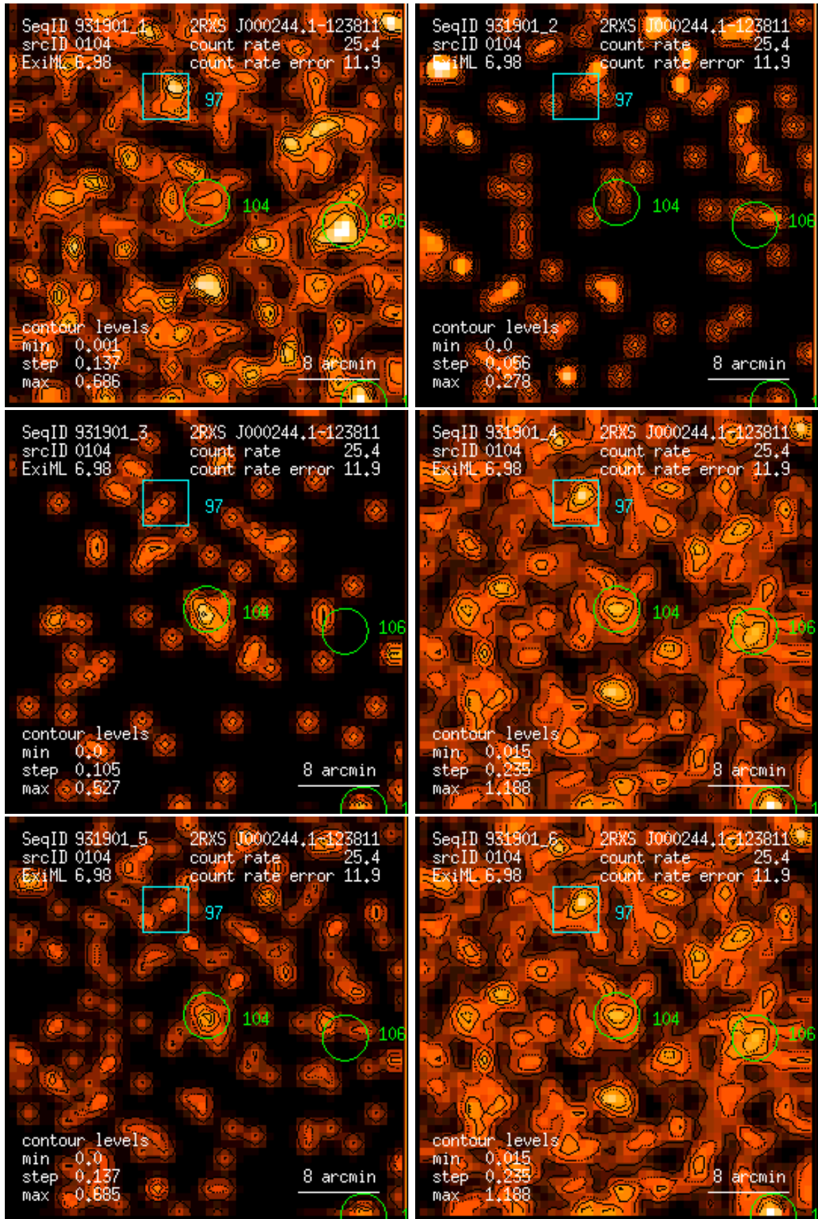
Figure 104: RASS 931901: detection 0104: band rate images, Gaussian filter: (1) PSPC channels 11 – 41, (2) 52 – 90, (3) 91 – 201, (4) 11 – 235, (5) 52 – 201, (6) 11 – 201. Broad band rates in counts/ks. Band rate contour levels in counts/ks/arcmin 2 .
