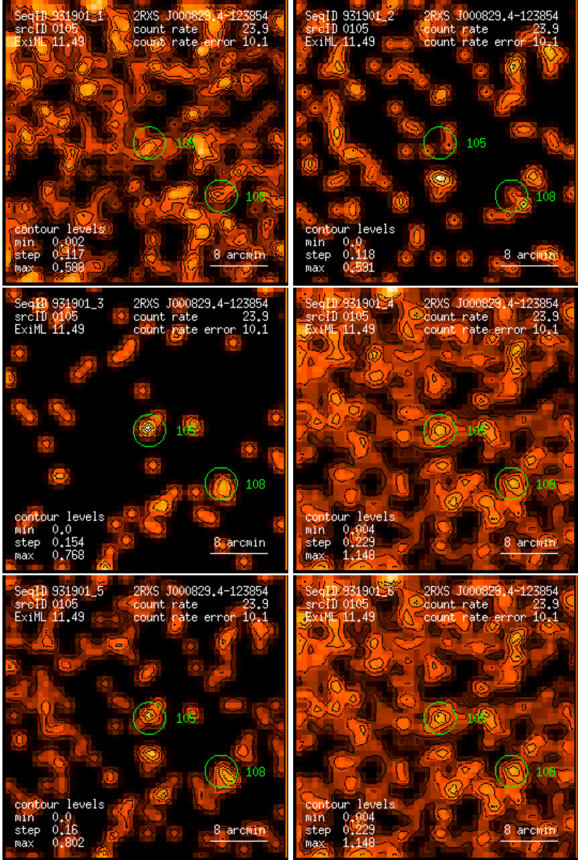
Figure 105: RASS 931901: detection 0105: band rate images, Gaussian filter: (1) PSPC channels 11 – 41, (2) 52 – 90, (3) 91 – 201, (4) 11 – 235, (5) 52 – 201, (6) 11 – 201. Broad band rates in counts/ks. Band rate contour levels in counts/ks/arcmin 2 .
