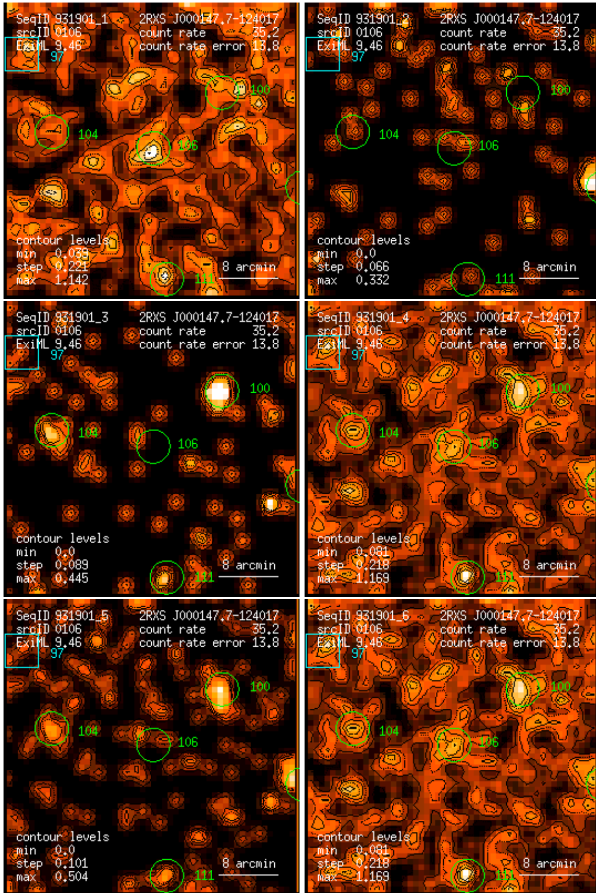
Figure 106: RASS 931901: detection 0106: band rate images, Gaussian filter: (1) PSPC channels 11 – 41, (2) 52 – 90, (3) 91 – 201, (4) 11 – 235, (5) 52 – 201, (6) 11 – 201. Broad band rates in counts/ks. Band rate contour levels in counts/ks/arcmin 2 .
