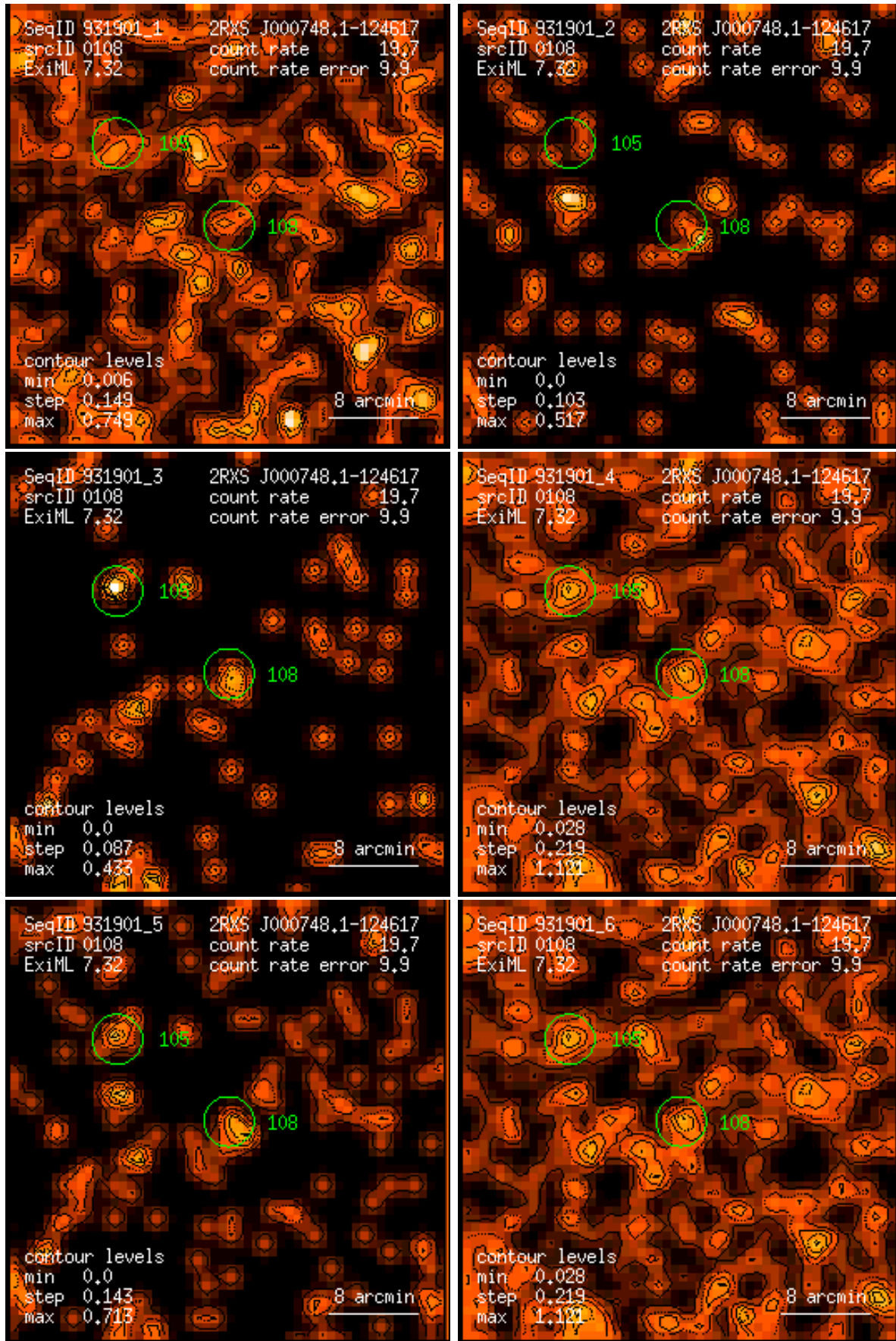
Figure 108: RASS 931901: detection 0108: band rate images, Gaussian filter: (1) PSPC channels 11 – 41, (2) 52 – 90, (3) 91 – 201, (4) 11 – 235, (5) 52 – 201, (6) 11 – 201. Broad band rates in counts/ks. Band rate contour levels in counts/ks/arcmin 2 .
