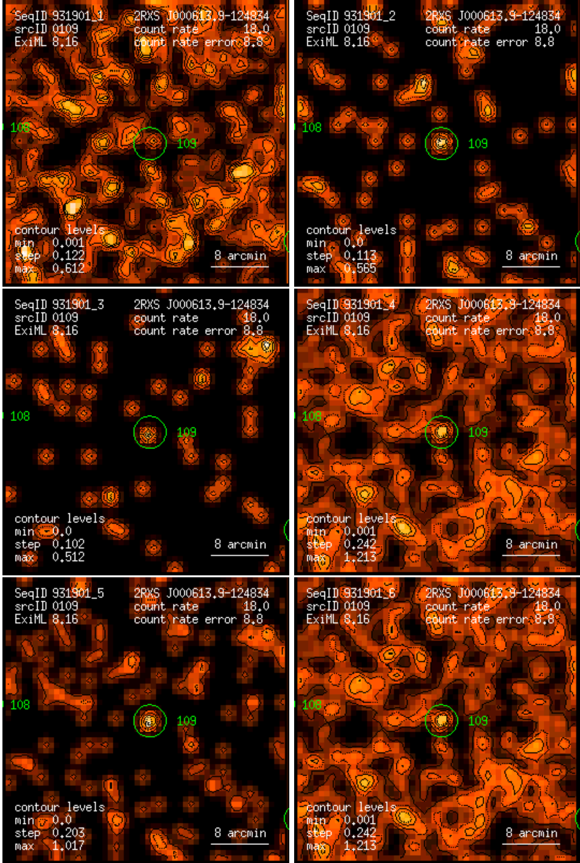
Figure 109: RASS 931901: detection 0109: band rate images, Gaussian filter: (1) PSPC channels 11 – 41, (2) 52 – 90, (3) 91 – 201, (4) 11 – 235, (5) 52 – 201, (6) 11 – 201. Broad band rates in counts/ks. Band rate contour levels in counts/ks/arcmin 2 .
