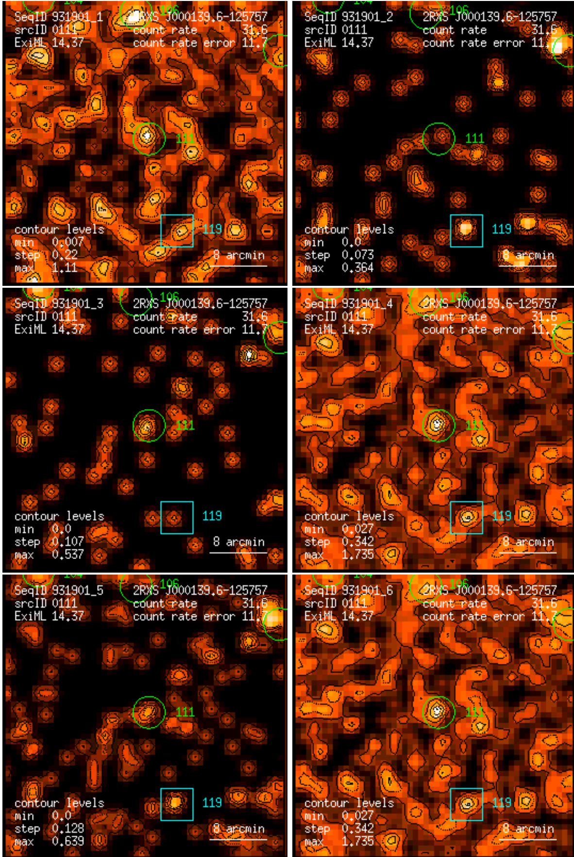
Figure 111: RASS 931901: detection 0111: band rate images, Gaussian filter: (1) PSPC channels 11 – 41, (2) 52 – 90, (3) 91 – 201, (4) 11 – 235, (5) 52 – 201, (6) 11 – 201. Broad band rates in counts/ks. Band rate contour levels in counts/ks/arcmin 2 .
