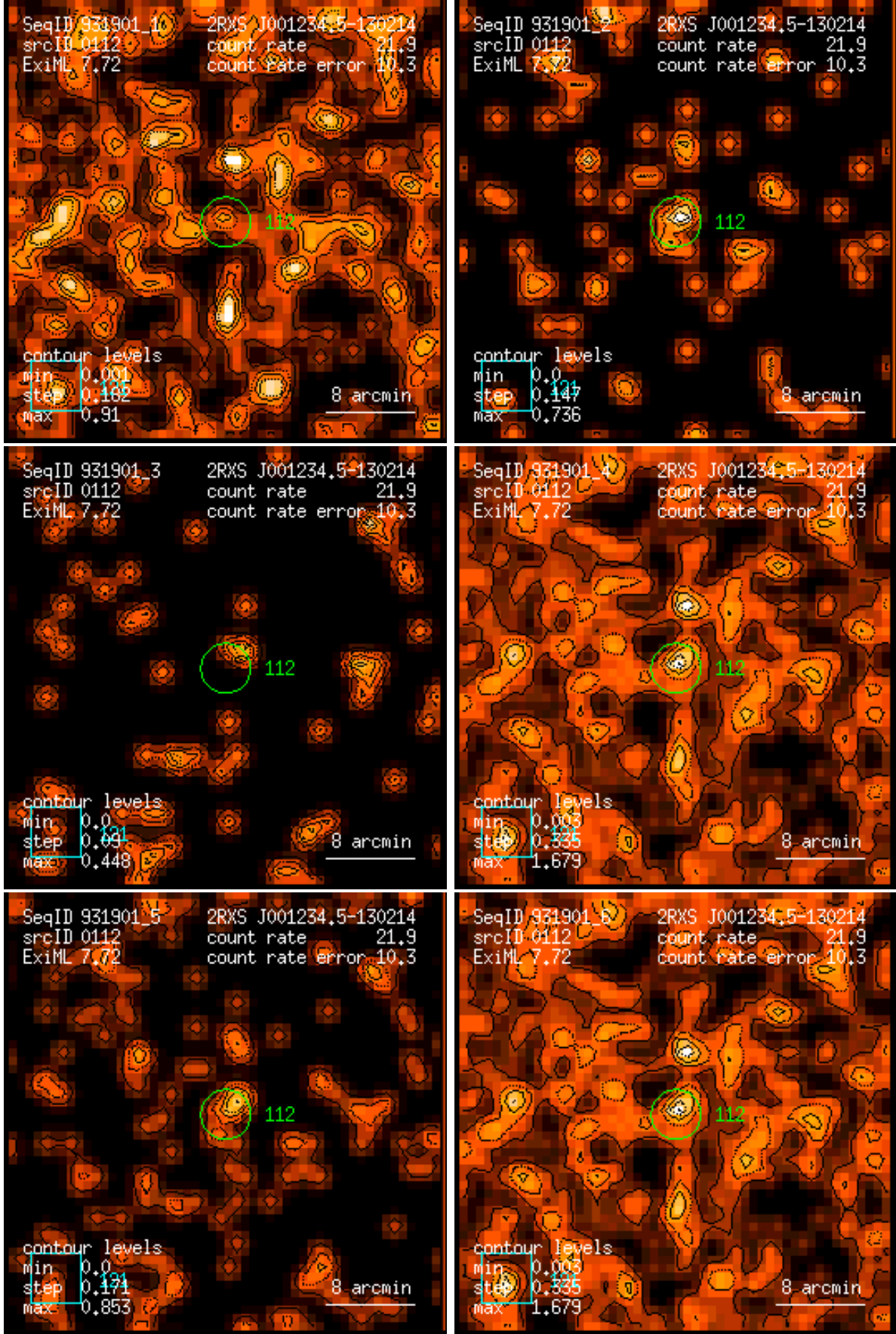
Figure 112: RASS 931901: detection 0112: band rate images, Gaussian filter: (1) PSPC channels 11 – 41, (2) 52 – 90, (3) 91 – 201, (4) 11 – 235, (5) 52 – 201, (6) 11 – 201. Broad band rates in counts/ks. Band rate contour levels in counts/ks/arcmin 2 .
