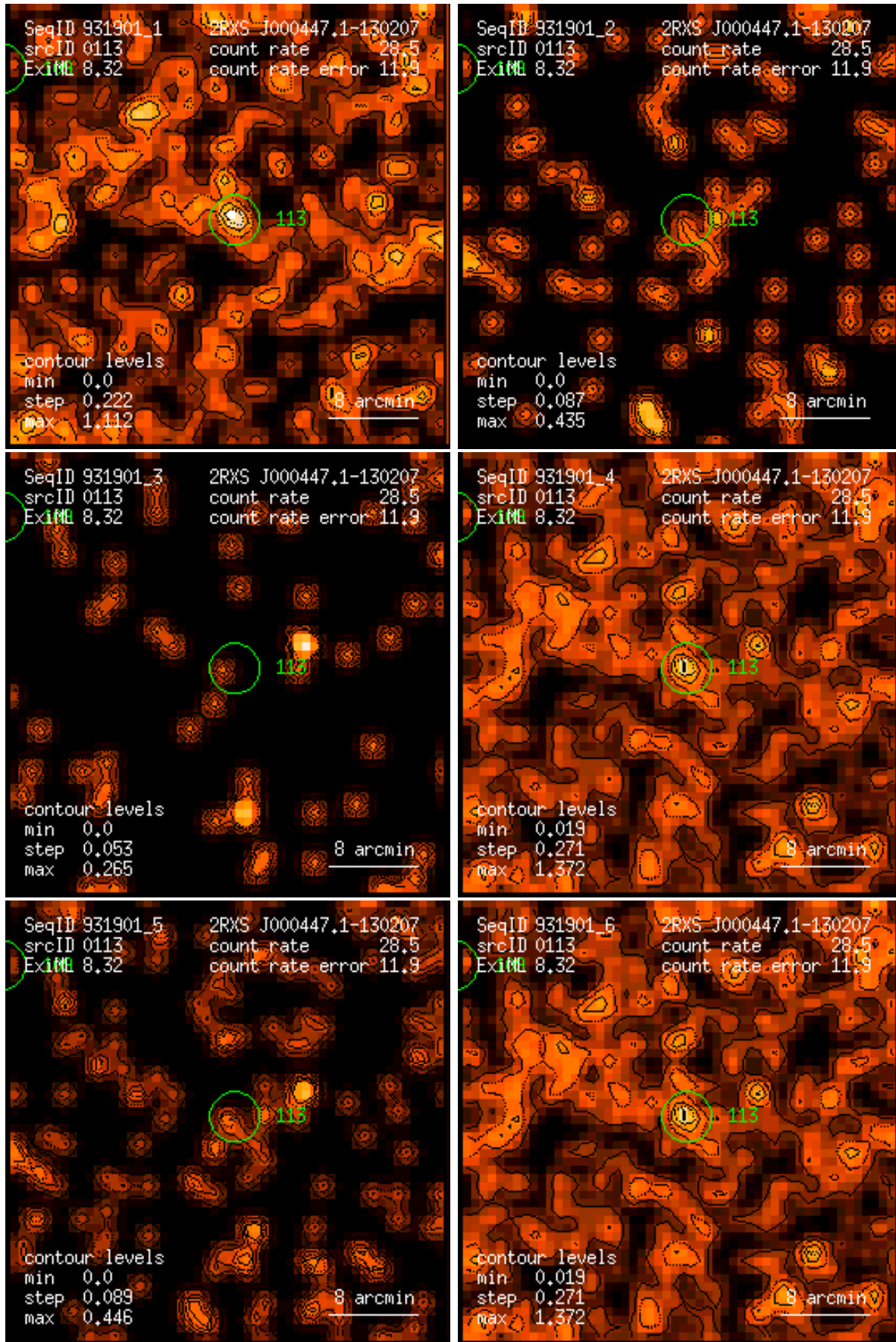
Figure 113: RASS 931901: detection 0113: band rate images, Gaussian filter: (1) PSPC channels 11 – 41, (2) 52 – 90, (3) 91 – 201, (4) 11 – 235, (5) 52 – 201, (6) 11 – 201. Broad band rates in counts/ks. Band rate contour levels in counts/ks/arcmin 2 .
