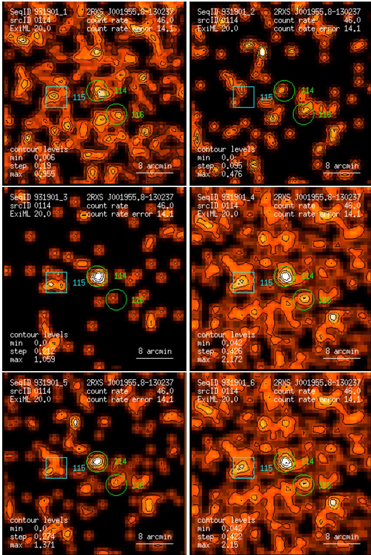
Figure 114: RASS 931901: detection 0114: band rate images, Gaussian filter: (1) PSPC channels 11 – 41, (2) 52 – 90, (3) 91 – 201, (4) 11 – 235, (5) 52 – 201, (6) 11 – 201. Broad band rates in counts/ks. Band rate contour levels in counts/ks/arcmin 2 .
