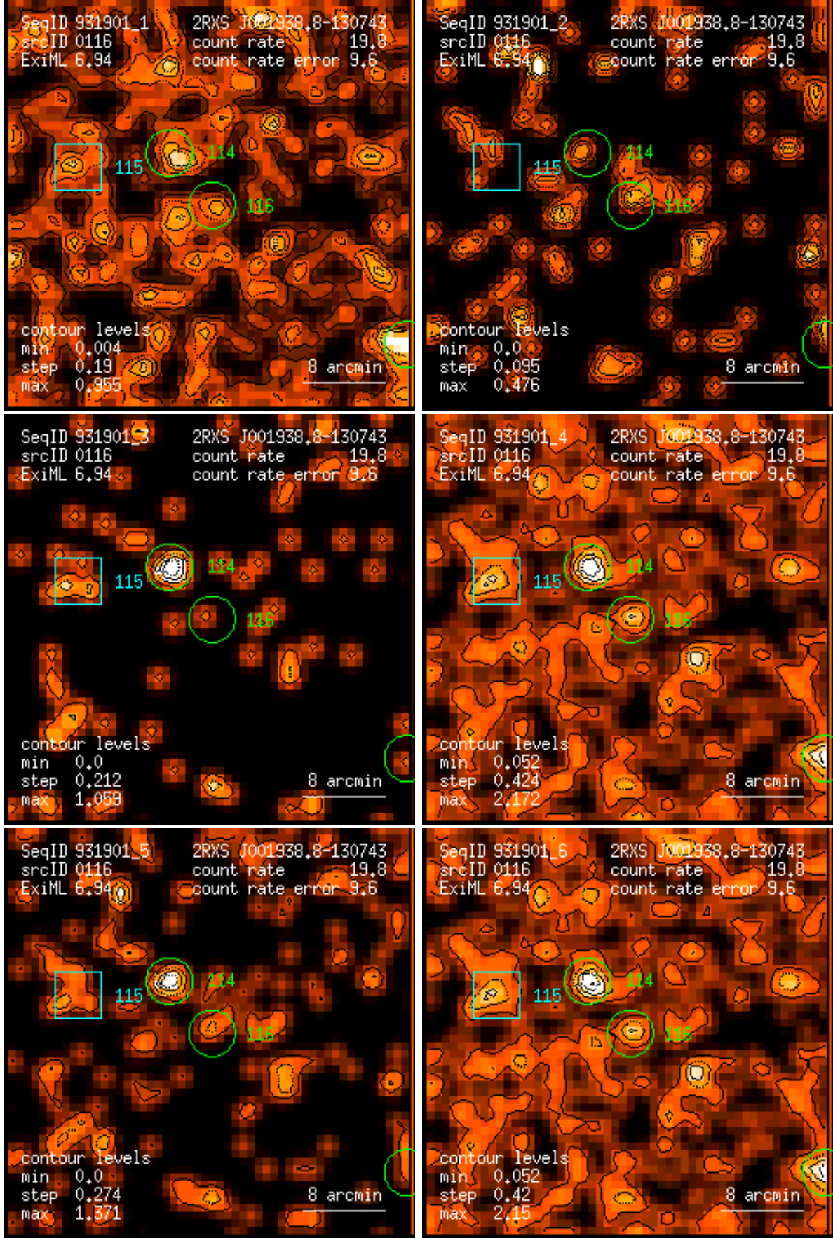
Figure 116: RASS 931901: detection 0116: band rate images, Gaussian filter: (1) PSPC channels 11 – 41, (2) 52 – 90, (3) 91 – 201, (4) 11 – 235, (5) 52 – 201, (6) 11 – 201. Broad band rates in counts/ks. Band rate contour levels in counts/ks/arcmin 2 .
