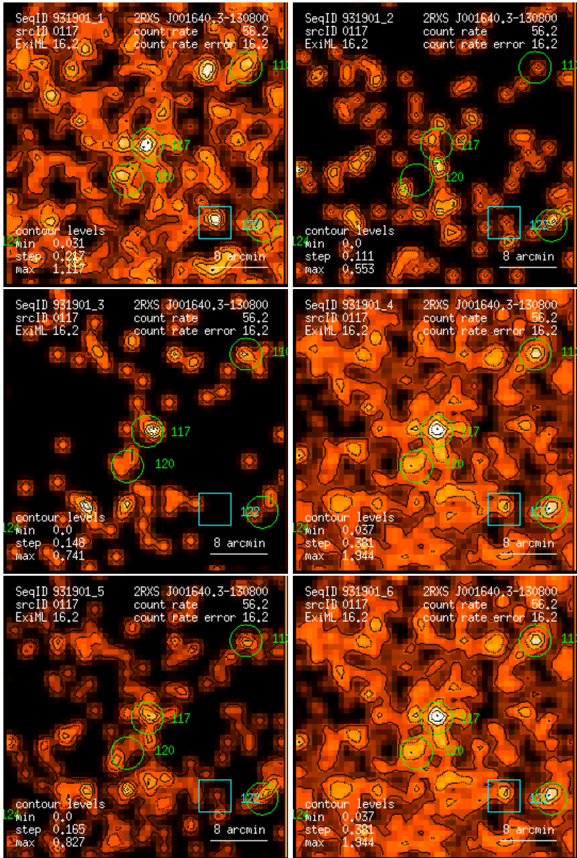
Figure 117: RASS 931901: detection 0117: band rate images, Gaussian filter: (1) PSPC channels 11 – 41, (2) 52 – 90, (3) 91 – 201, (4) 11 – 235, (5) 52 – 201, (6) 11 – 201. Broad band rates in counts/ks. Band rate contour levels in counts/ks/arcmin 2 .
