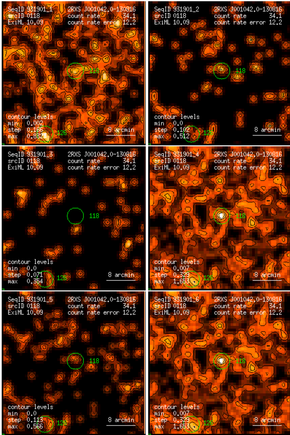
Figure 118: RASS 931901: detection 0118: band rate images, Gaussian filter: (1) PSPC channels 11 – 41, (2) 52 – 90, (3) 91 – 201, (4) 11 – 235, (5) 52 – 201, (6) 11 – 201. Broad band rates in counts/ks. Band rate contour levels in counts/ks/arcmin 2 .
