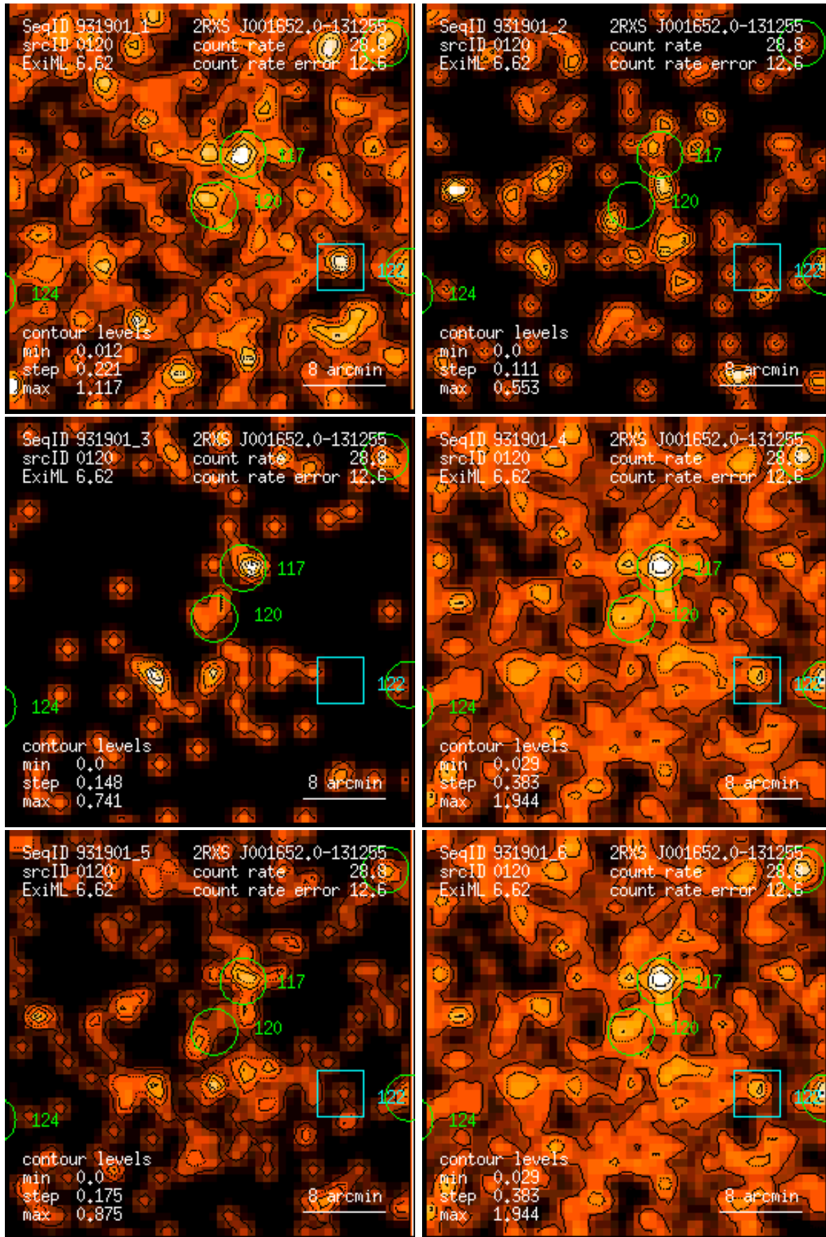
Figure 120: RASS 931901: detection 0120: band rate images, Gaussian filter: (1) PSPC channels 11 – 41, (2) 52 – 90, (3) 91 – 201, (4) 11 – 235, (5) 52 – 201, (6) 11 – 201. Broad band rates in counts/ks. Band rate contour levels in counts/ks/arcmin 2 .
