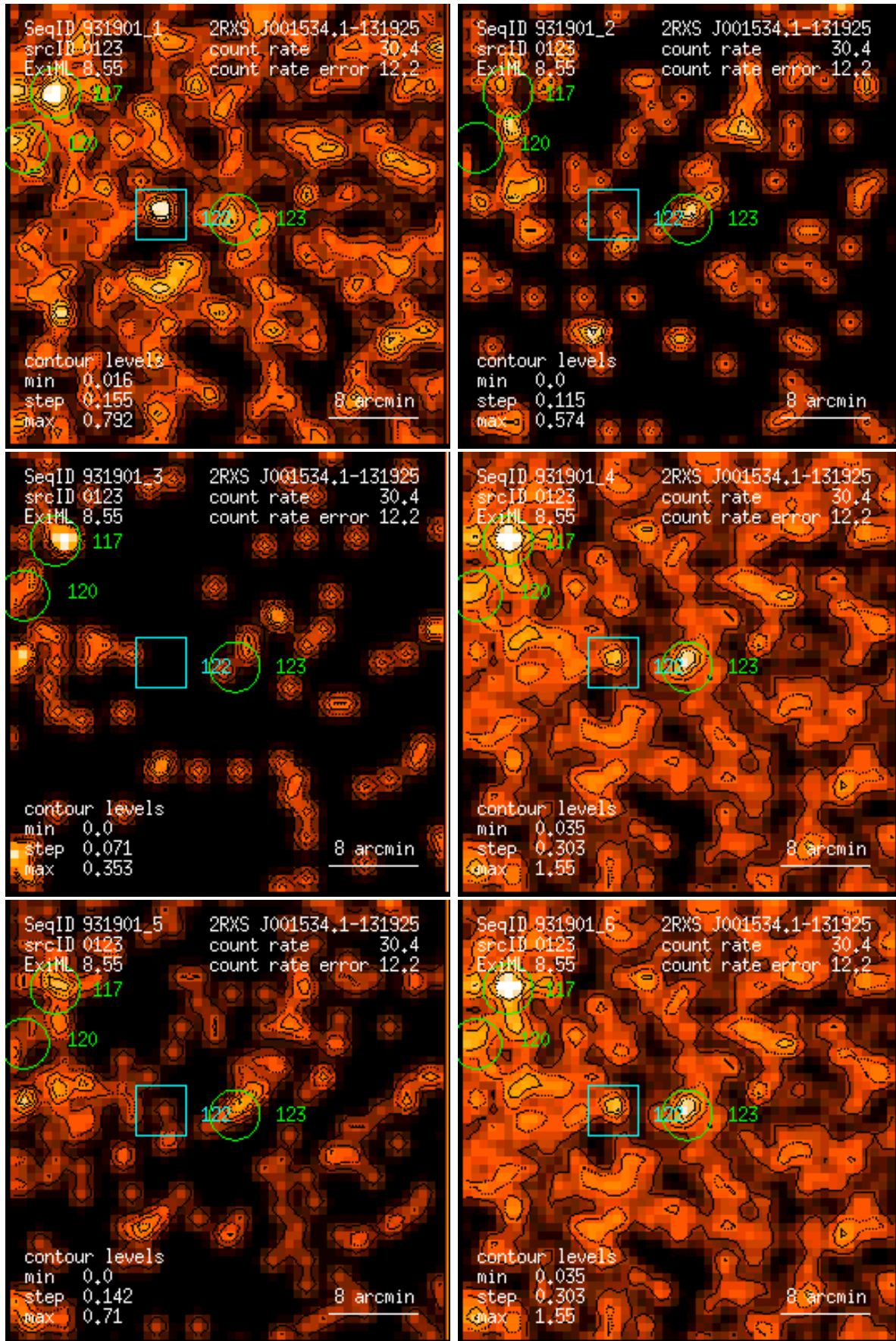
Figure 123: RASS 931901: detection 0123: band rate images, Gaussian filter: (1) PSPC channels 11 – 41, (2) 52 – 90, (3) 91 – 201, (4) 11 – 235, (5) 52 – 201, (6) 11 – 201. Broad band rates in counts/ks. Band rate contour levels in counts/ks/arcmin 2 .
