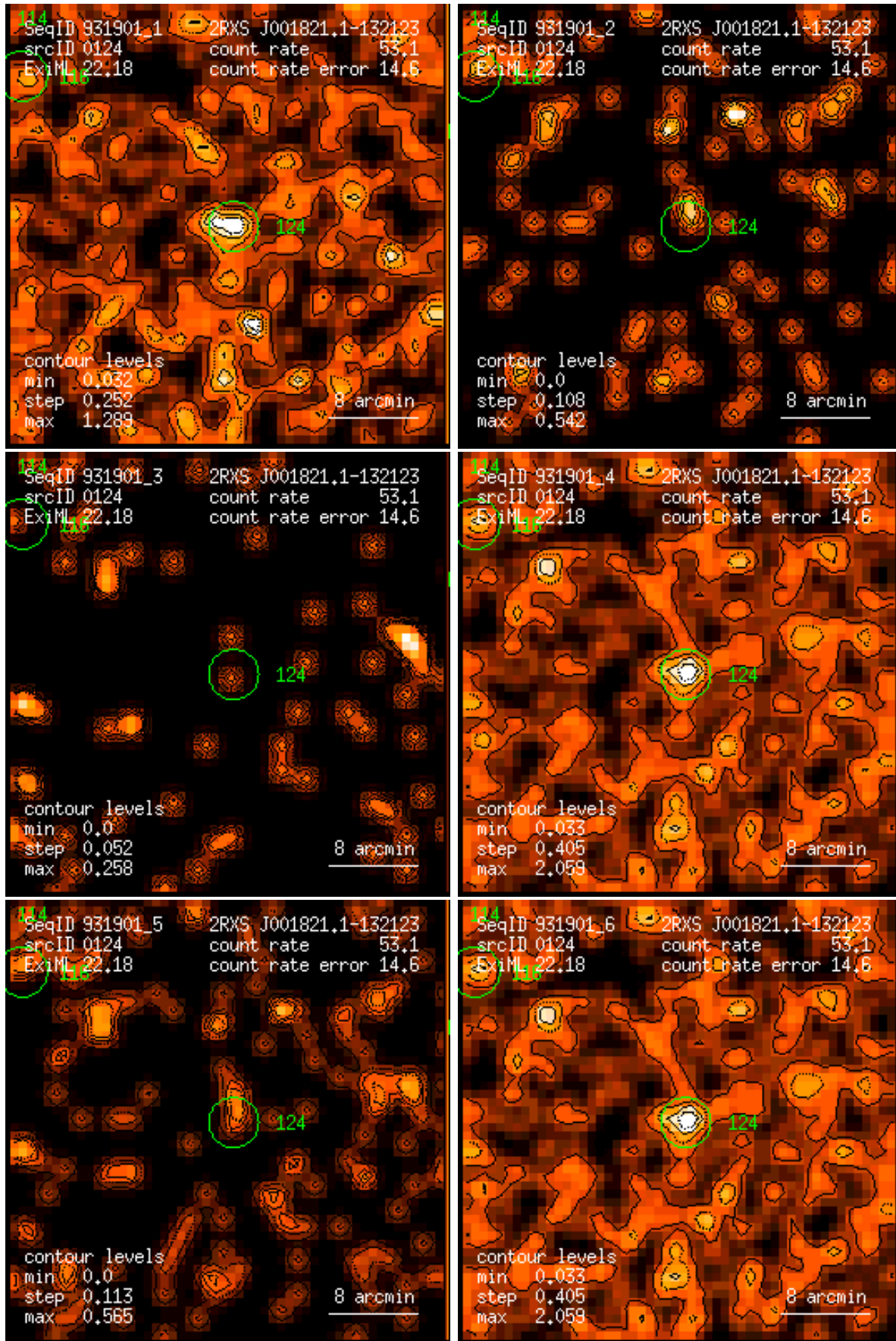
Figure 124: RASS 931901: detection 0124: band rate images, Gaussian filter: (1) PSPC channels 11 – 41, (2) 52 – 90, (3) 91 – 201, (4) 11 – 235, (5) 52 – 201, (6) 11 – 201. Broad band rates in counts/ks. Band rate contour levels in counts/ks/arcmin 2 .
