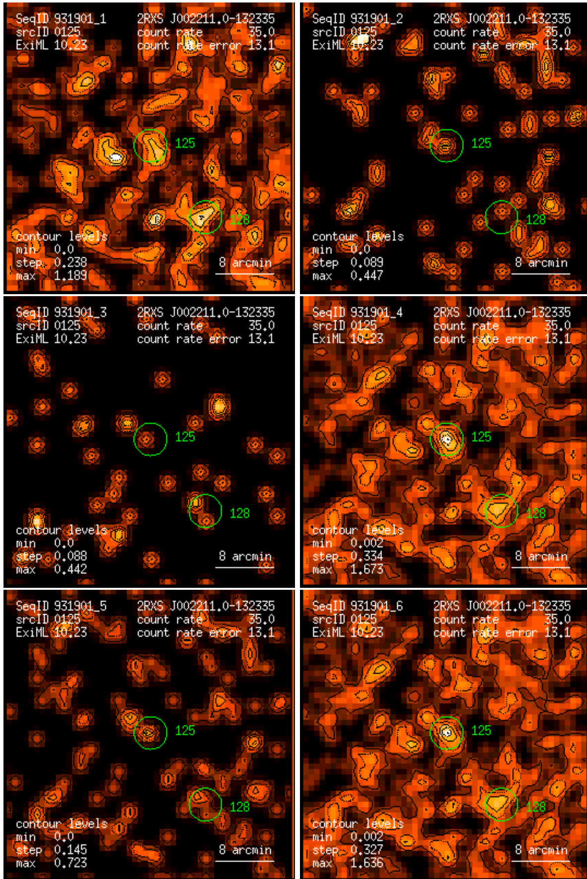
Figure 125: RASS 931901: detection 0125: band rate images, Gaussian filter: (1) PSPC channels 11 – 41, (2) 52 – 90, (3) 91 – 201, (4) 11 – 235, (5) 52 – 201, (6) 11 – 201. Broad band rates in counts/ks. Band rate contour levels in counts/ks/arcmin 2 .
