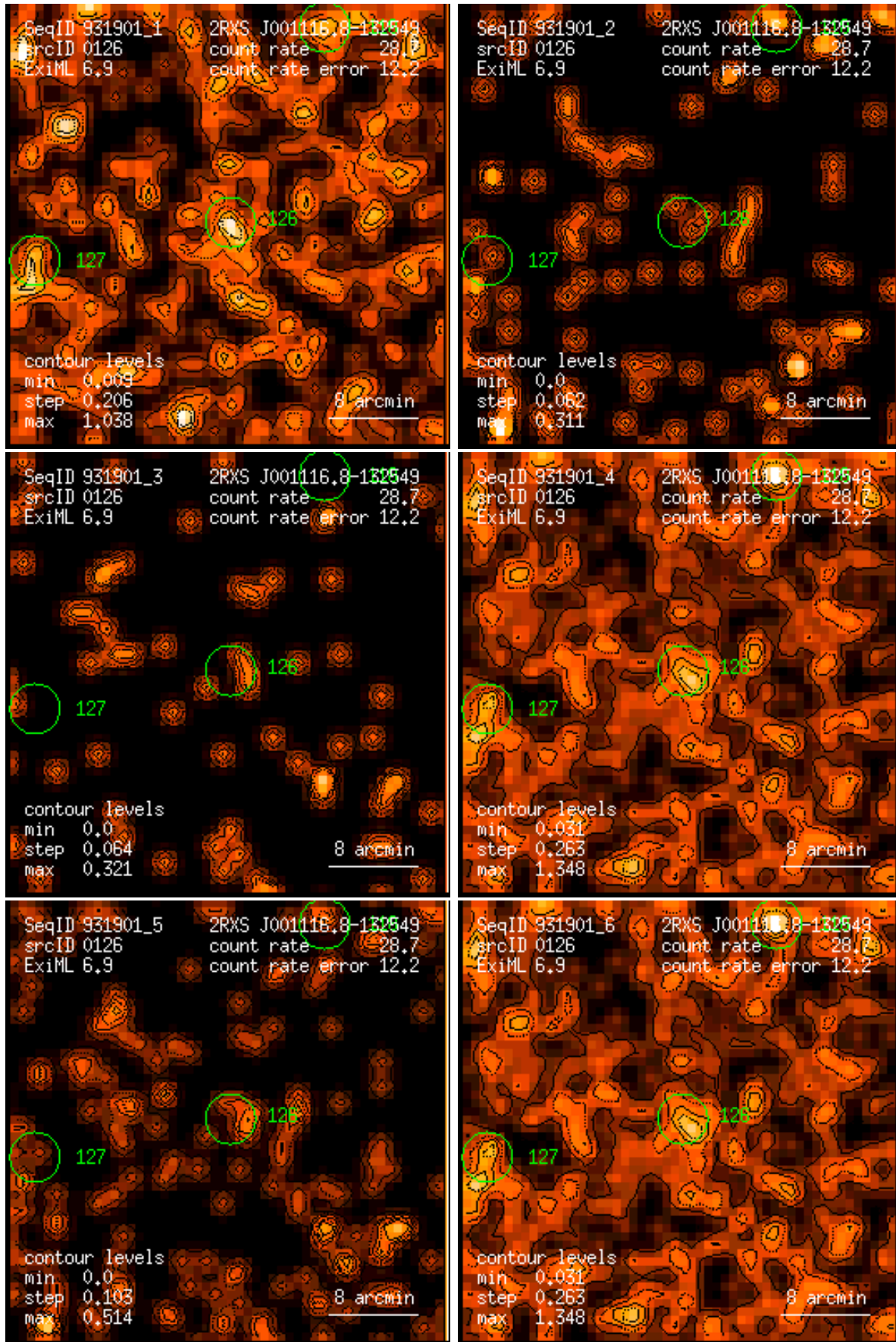
Figure 126: RASS 931901: detection 0126: band rate images, Gaussian filter: (1) PSPC channels 11 – 41, (2) 52 – 90, (3) 91 – 201, (4) 11 – 235, (5) 52 – 201, (6) 11 – 201. Broad band rates in counts/ks. Band rate contour levels in counts/ks/arcmin 2 .
