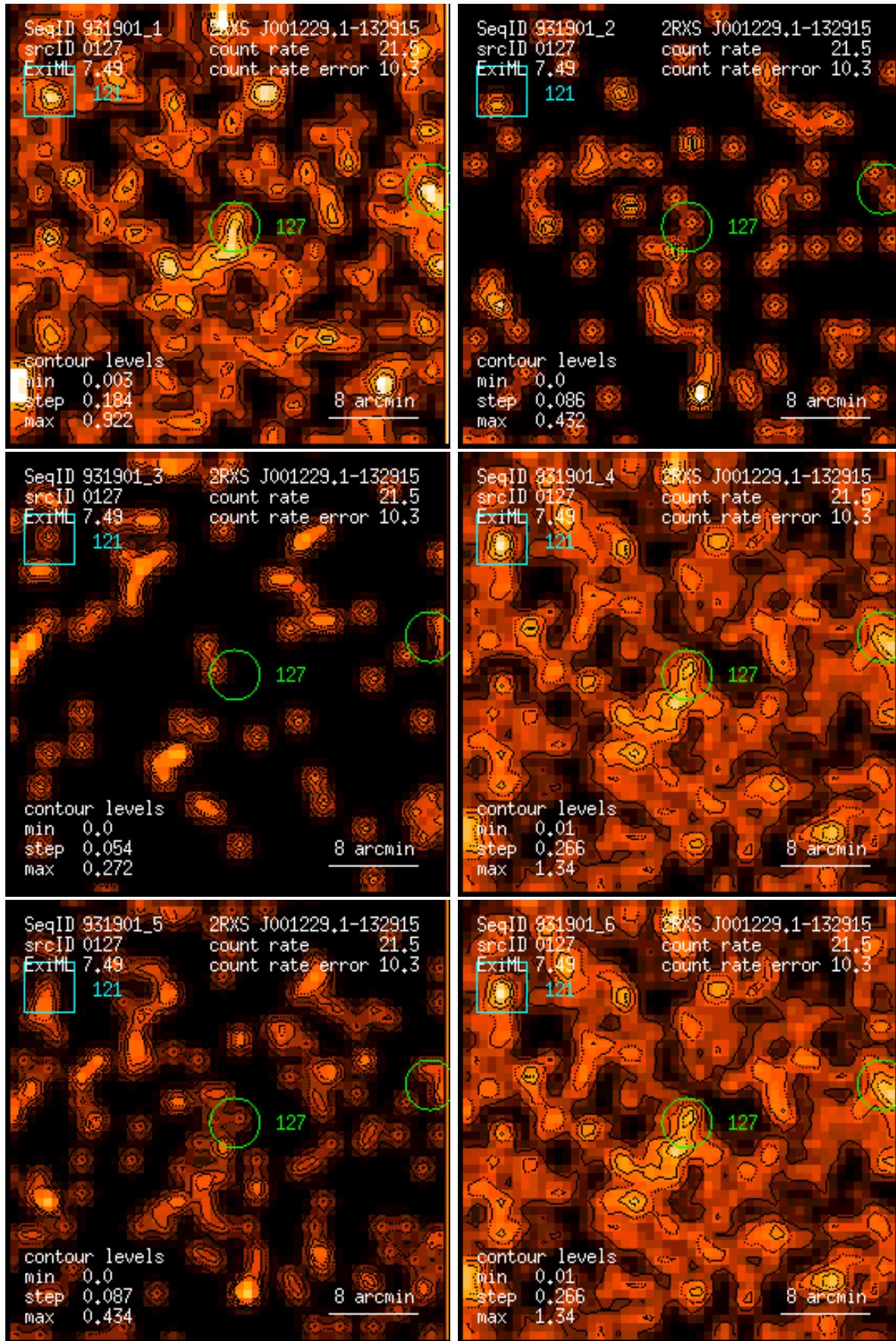
Figure 127: RASS 931901: detection 0127: band rate images, Gaussian filter: (1) PSPC channels 11 – 41, (2) 52 – 90, (3) 91 – 201, (4) 11 – 235, (5) 52 – 201, (6) 11 – 201. Broad band rates in counts/ks. Band rate contour levels in counts/ks/arcmin 2 .
