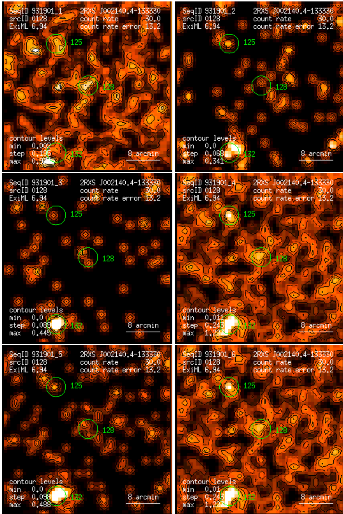
Figure 128: RASS 931901: detection 0128: band rate images, Gaussian filter: (1) PSPC channels 11 – 41, (2) 52 – 90, (3) 91 – 201, (4) 11 – 235, (5) 52 – 201, (6) 11 – 201. Broad band rates in counts/ks. Band rate contour levels in counts/ks/arcmin 2 .
