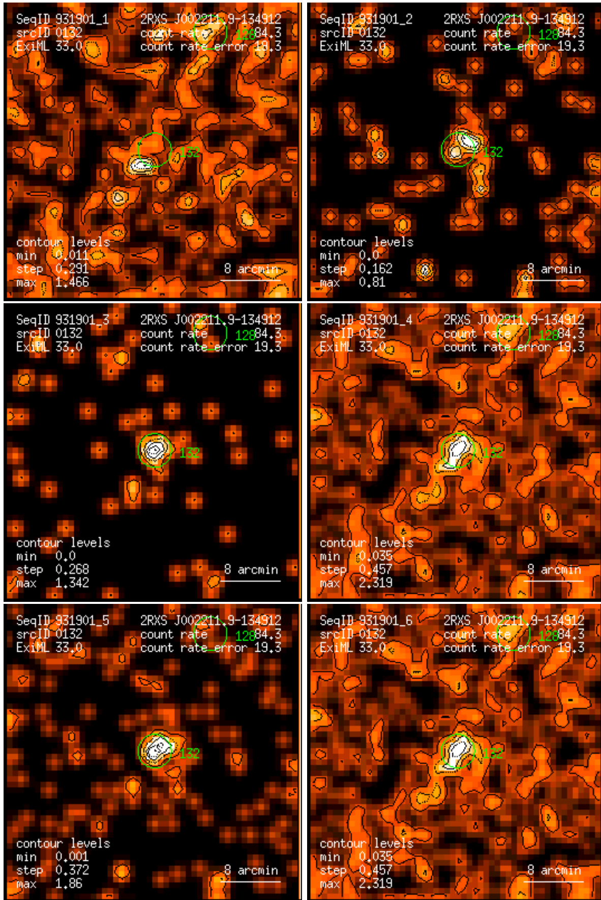
Figure 132: RASS 931901: detection 0132: band rate images, Gaussian filter: (1) PSPC channels 11 – 41, (2) 52 – 90, (3) 91 – 201, (4) 11 – 235, (5) 52 – 201, (6) 11 – 201. Broad band rates in counts/ks. Band rate contour levels in counts/ks/arcmin 2 .
