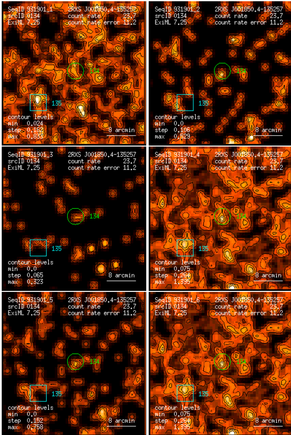
Figure 134: RASS 931901: detection 0134: band rate images, Gaussian filter: (1) PSPC channels 11 – 41, (2) 52 – 90, (3) 91 – 201, (4) 11 – 235, (5) 52 – 201, (6) 11 – 201. Broad band rates in counts/ks. Band rate contour levels in counts/ks/arcmin 2 .
