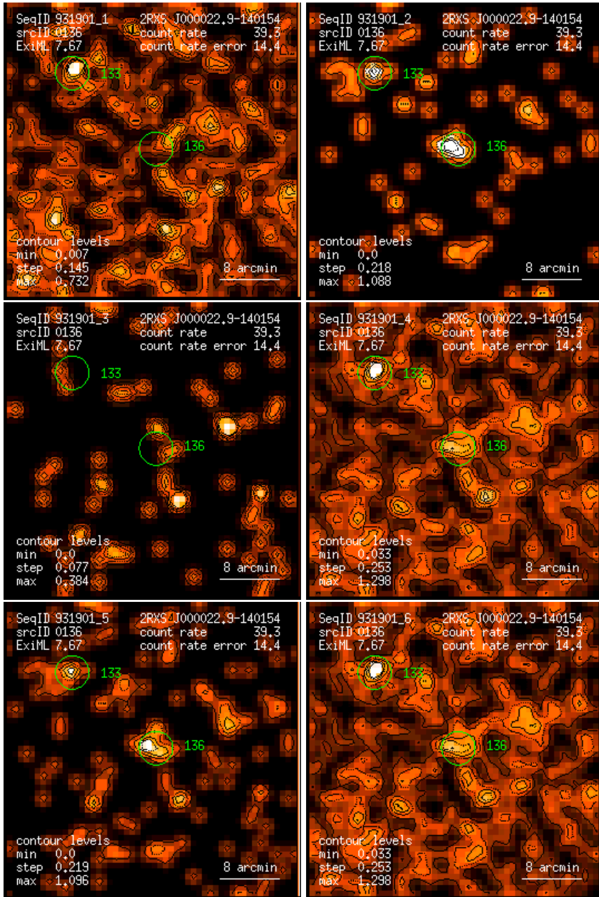
Figure 136: RASS 931901: detection 0136: band rate images, Gaussian filter: (1) PSPC channels 11 – 41, (2) 52 – 90, (3) 91 – 201, (4) 11 – 235, (5) 52 – 201, (6) 11 – 201. Broad band rates in counts/ks. Band rate contour levels in counts/ks/arcmin 2 .
