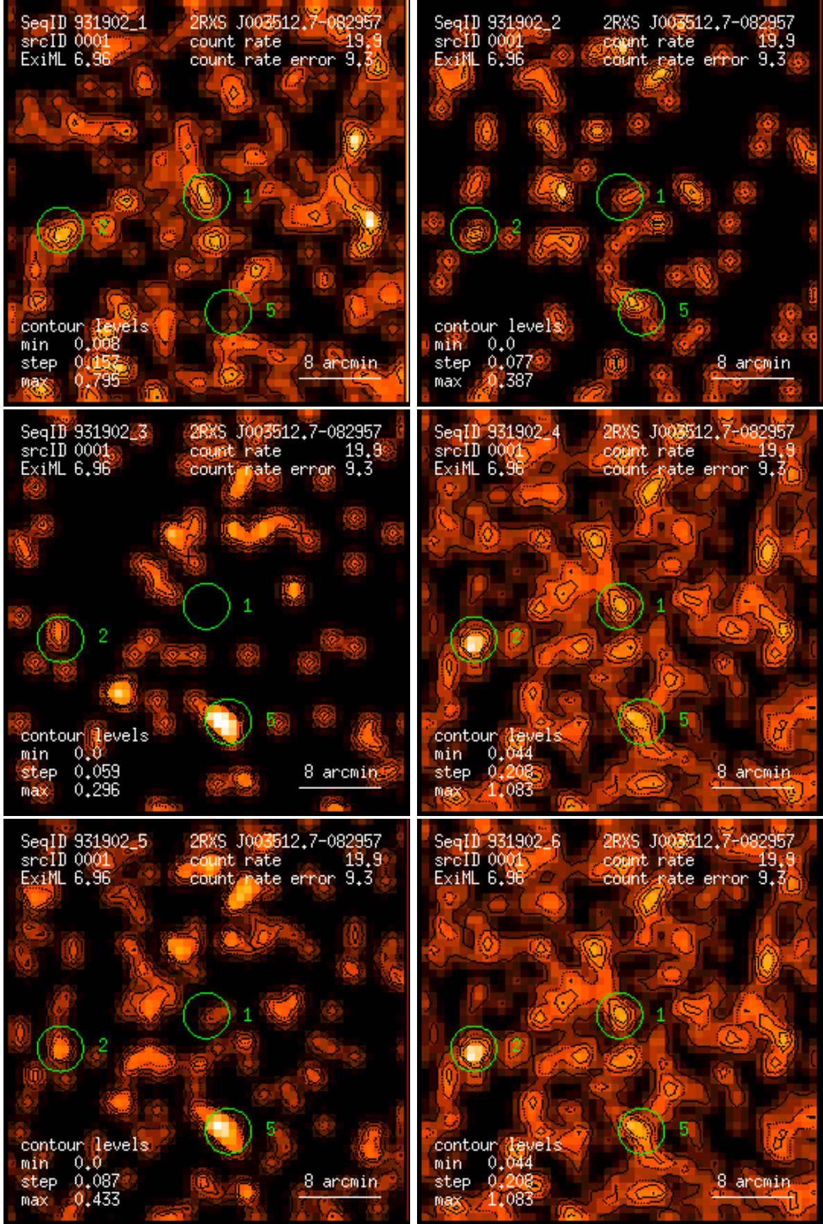
Figure 1: RASS 931902: detection 0001: band rate images, Gaussian filter: (1) PSPC channels 11 – 41, (2) 52 – 90, (3) 91 – 201, (4) 11 – 235, (5) 52 – 201, (6) 11 – 201. Broad band rates in counts/ks. Band rate contour levels in counts/ks/arcmin 2 .
