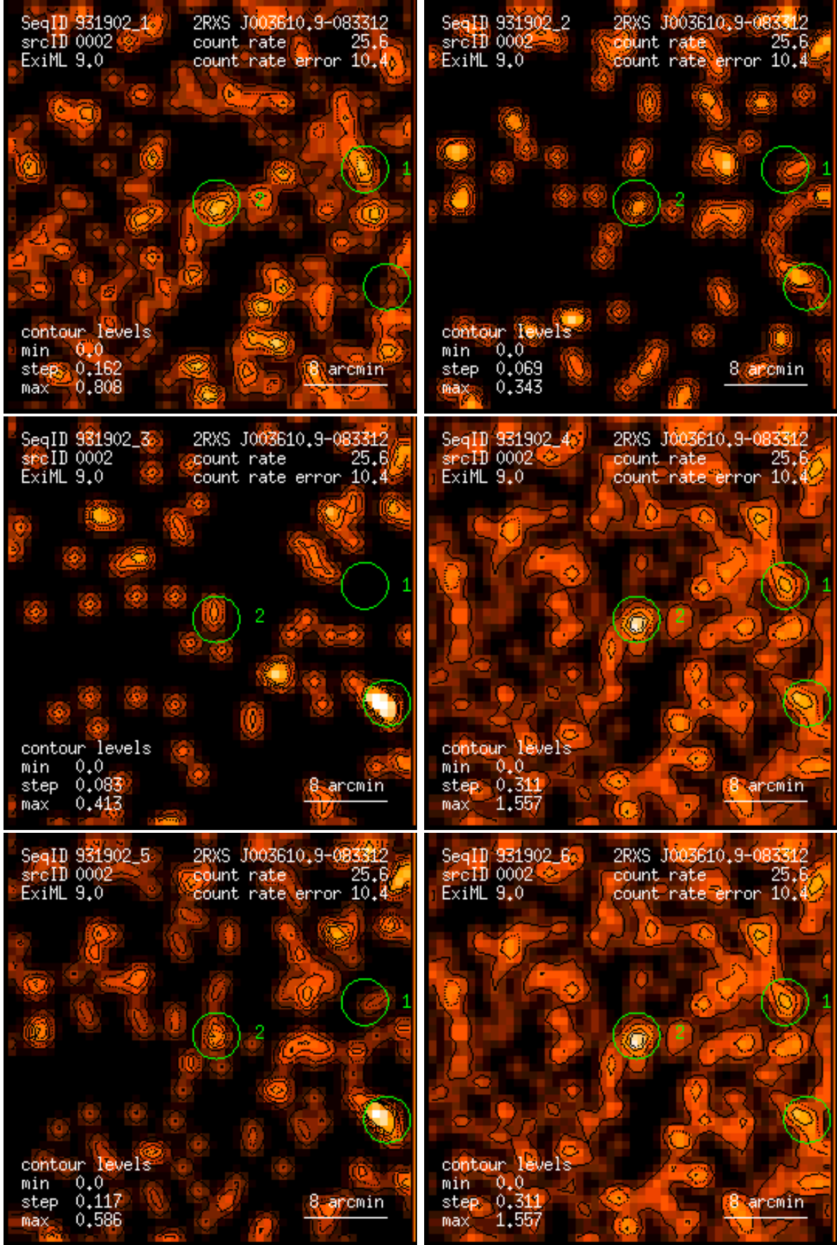
Figure 2: RASS 931902: detection 0002: band rate images, Gaussian filter: (1) PSPC channels 11 – 41, (2) 52 – 90, (3) 91 – 201, (4) 11 – 235, (5) 52 – 201, (6) 11 – 201. Broad band rates in counts/ks. Band rate contour levels in counts/ks/arcmin 2 .
