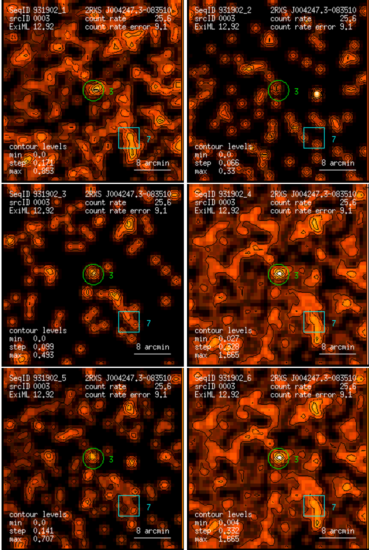
Figure 3: RASS 931902: detection 0003: band rate images, Gaussian filter: (1) PSPC channels 11 – 41, (2) 52 – 90, (3) 91 – 201, (4) 11 – 235, (5) 52 – 201, (6) 11 – 201. Broad band rates in counts/ks. Band rate contour levels in counts/ks/arcmin 2 .
