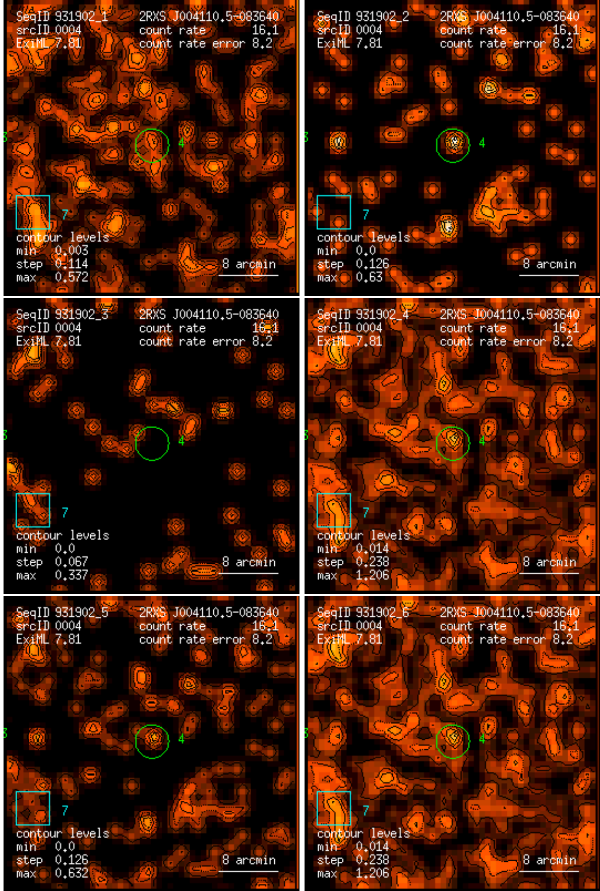
Figure 4: RASS 931902: detection 0004: band rate images, Gaussian filter: (1) PSPC channels 11 – 41, (2) 52 – 90, (3) 91 – 201, (4) 11 – 235, (5) 52 – 201, (6) 11 – 201. Broad band rates in counts/ks. Band rate contour levels in counts/ks/arcmin 2 .
