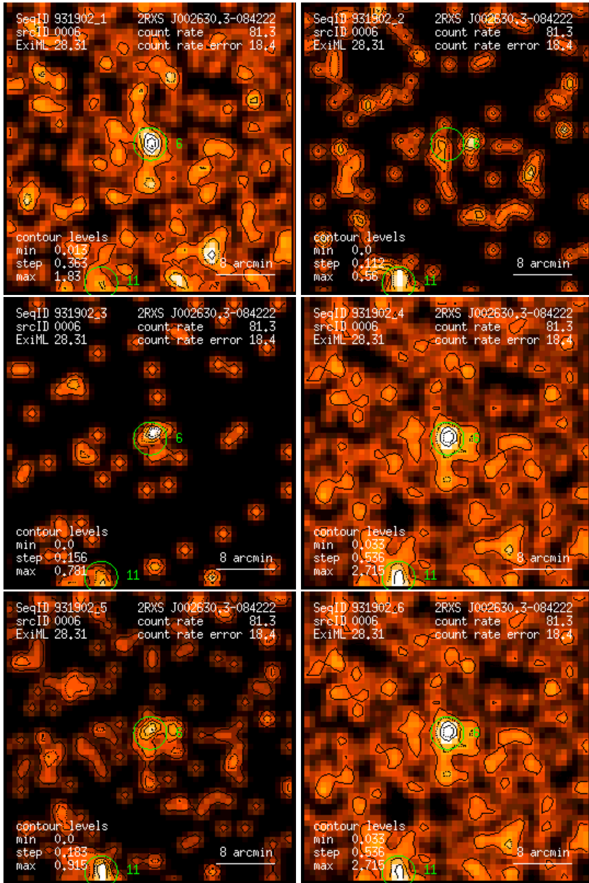
Figure 6: RASS 931902: detection 0006: band rate images, Gaussian filter: (1) PSPC channels 11 – 41, (2) 52 – 90, (3) 91 – 201, (4) 11 – 235, (5) 52 – 201, (6) 11 – 201. Broad band rates in counts/ks. Band rate contour levels in counts/ks/arcmin 2 .
