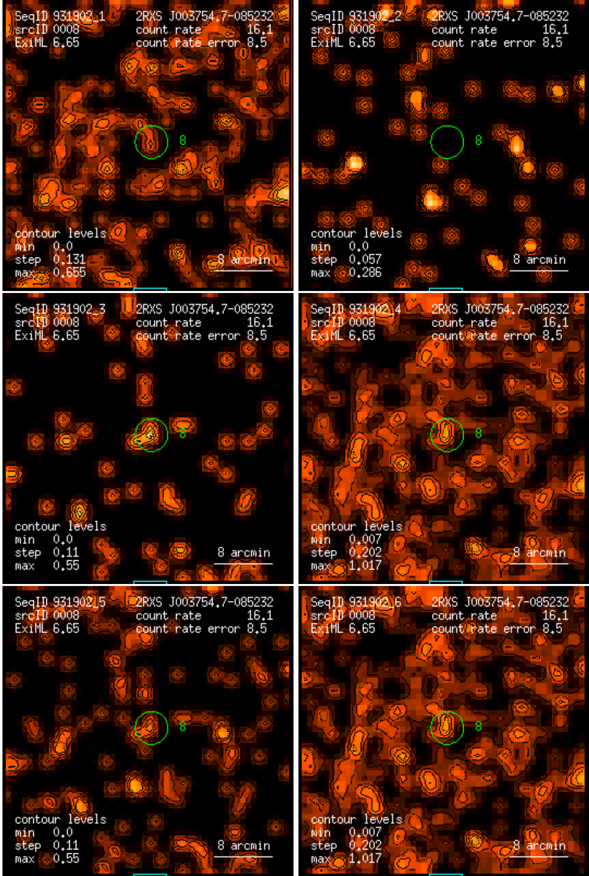
Figure 8: RASS 931902: detection 0008: band rate images, Gaussian filter: (1) PSPC channels 11 – 41, (2) 52 – 90, (3) 91 – 201, (4) 11 – 235, (5) 52 – 201, (6) 11 – 201. Broad band rates in counts/ks. Band rate contour levels in counts/ks/arcmin 2 .
