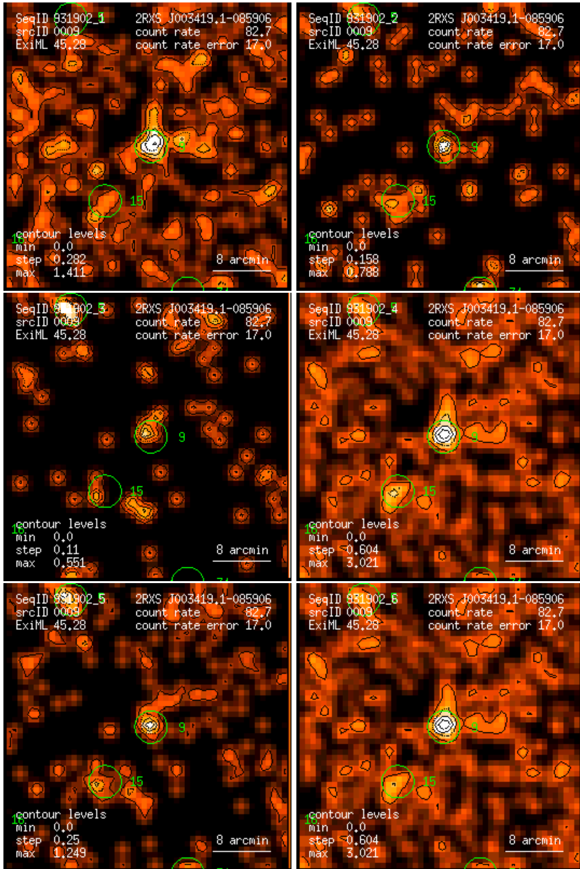
Figure 9: RASS 931902: detection 0009: band rate images, Gaussian filter: (1) PSPC channels 11 – 41, (2) 52 – 90, (3) 91 – 201, (4) 11 – 235, (5) 52 – 201, (6) 11 – 201. Broad band rates in counts/ks. Band rate contour levels in counts/ks/arcmin 2 .
