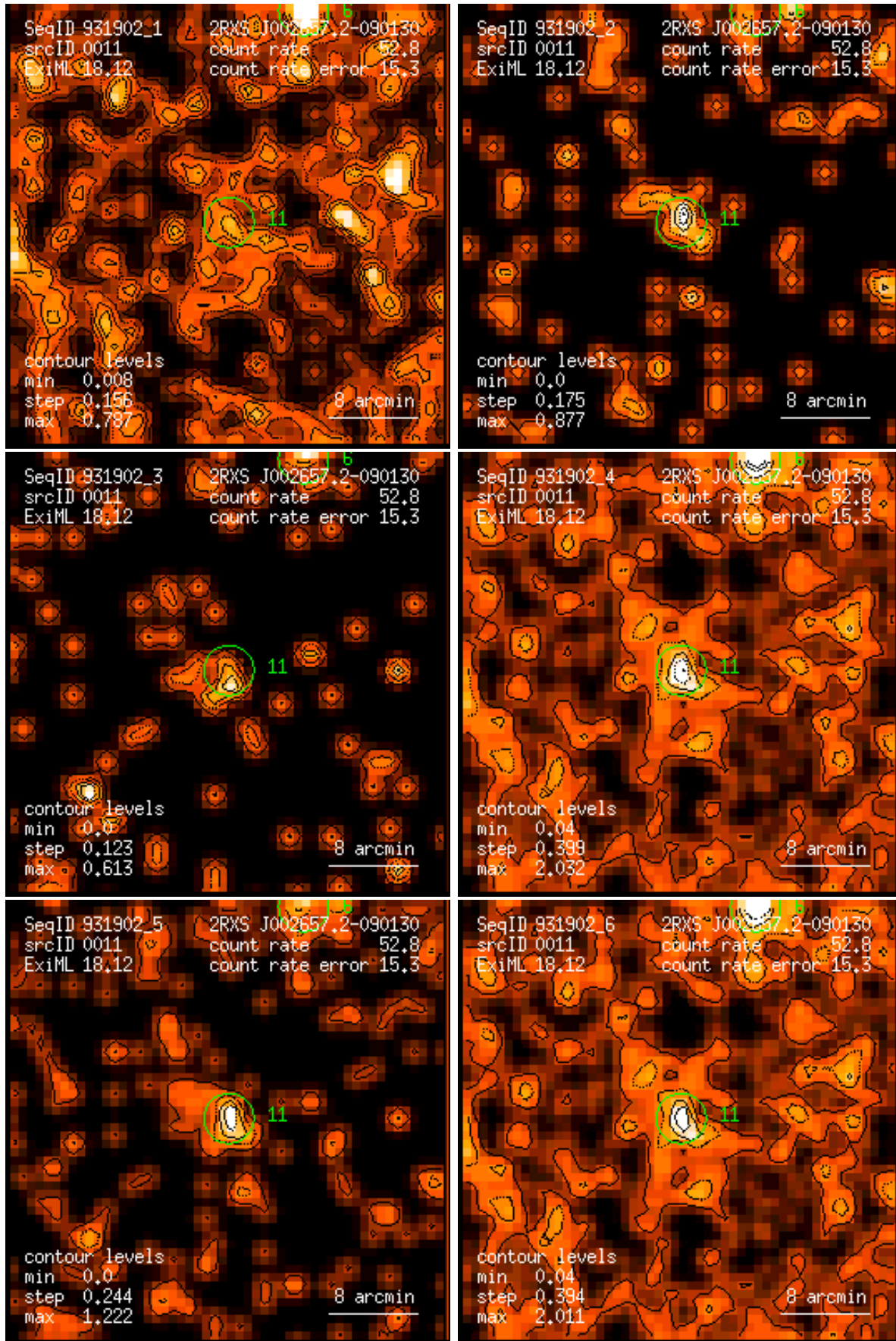
Figure 11: RASS 931902: detection 0011: band rate images, Gaussian filter: (1) PSPC channels 11 – 41, (2) 52 – 90, (3) 91 – 201, (4) 11 – 235, (5) 52 – 201, (6) 11 – 201. Broad band rates in counts/ks. Band rate contour levels in counts/ks/arcmin 2 .
