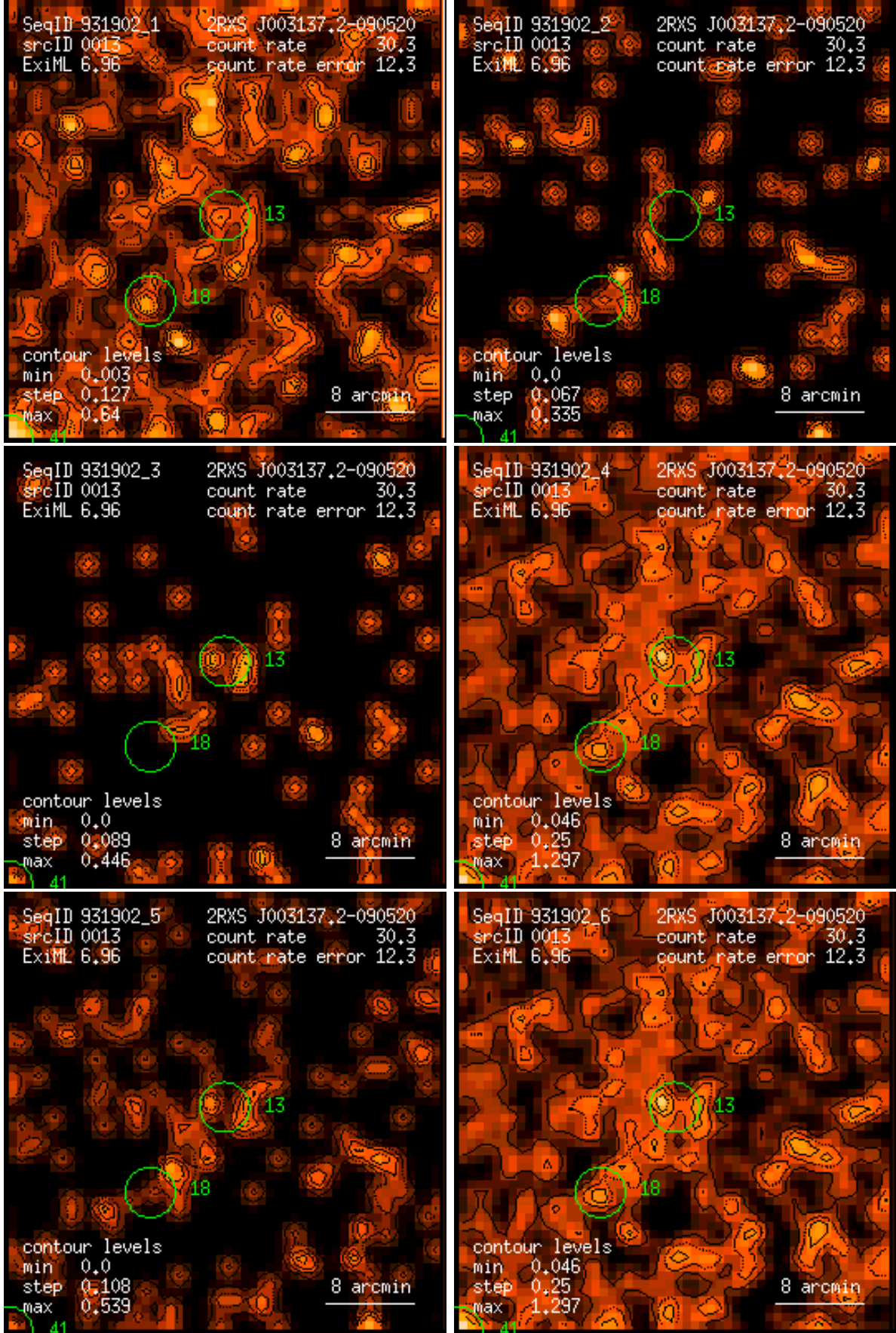
Figure 13: RASS 931902: detection 0013: band rate images, Gaussian filter: (1) PSPC channels 11 – 41, (2) 52 – 90, (3) 91 – 201, (4) 11 – 235, (5) 52 – 201, (6) 11 – 201. Broad band rates in counts/ks. Band rate contour levels in counts/ks/arcmin 2 .
