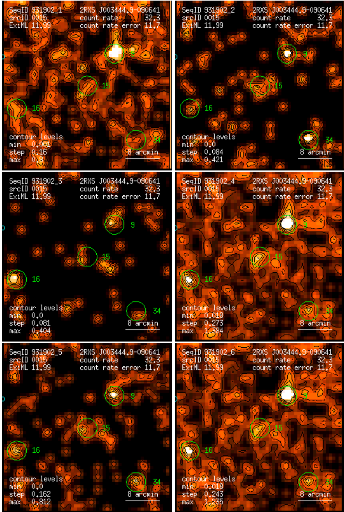
Figure 15: RASS 931902: detection 0015: band rate images, Gaussian filter: (1) PSPC channels 11 – 41, (2) 52 – 90, (3) 91 – 201, (4) 11 – 235, (5) 52 – 201, (6) 11 – 201. Broad band rates in counts/ks. Band rate contour levels in counts/ks/arcmin 2 .
