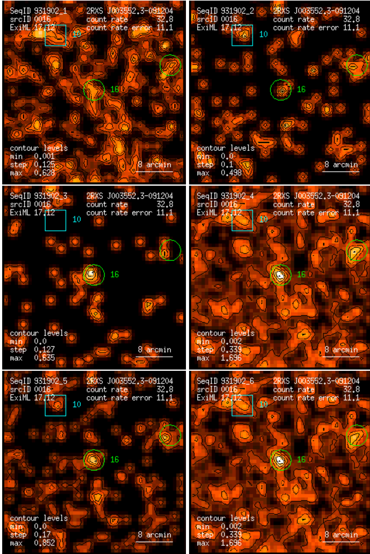
Figure 16: RASS 931902: detection 0016: band rate images, Gaussian filter: (1) PSPC channels 11 – 41, (2) 52 – 90, (3) 91 – 201, (4) 11 – 235, (5) 52 – 201, (6) 11 – 201. Broad band rates in counts/ks. Band rate contour levels in counts/ks/arcmin 2 .
