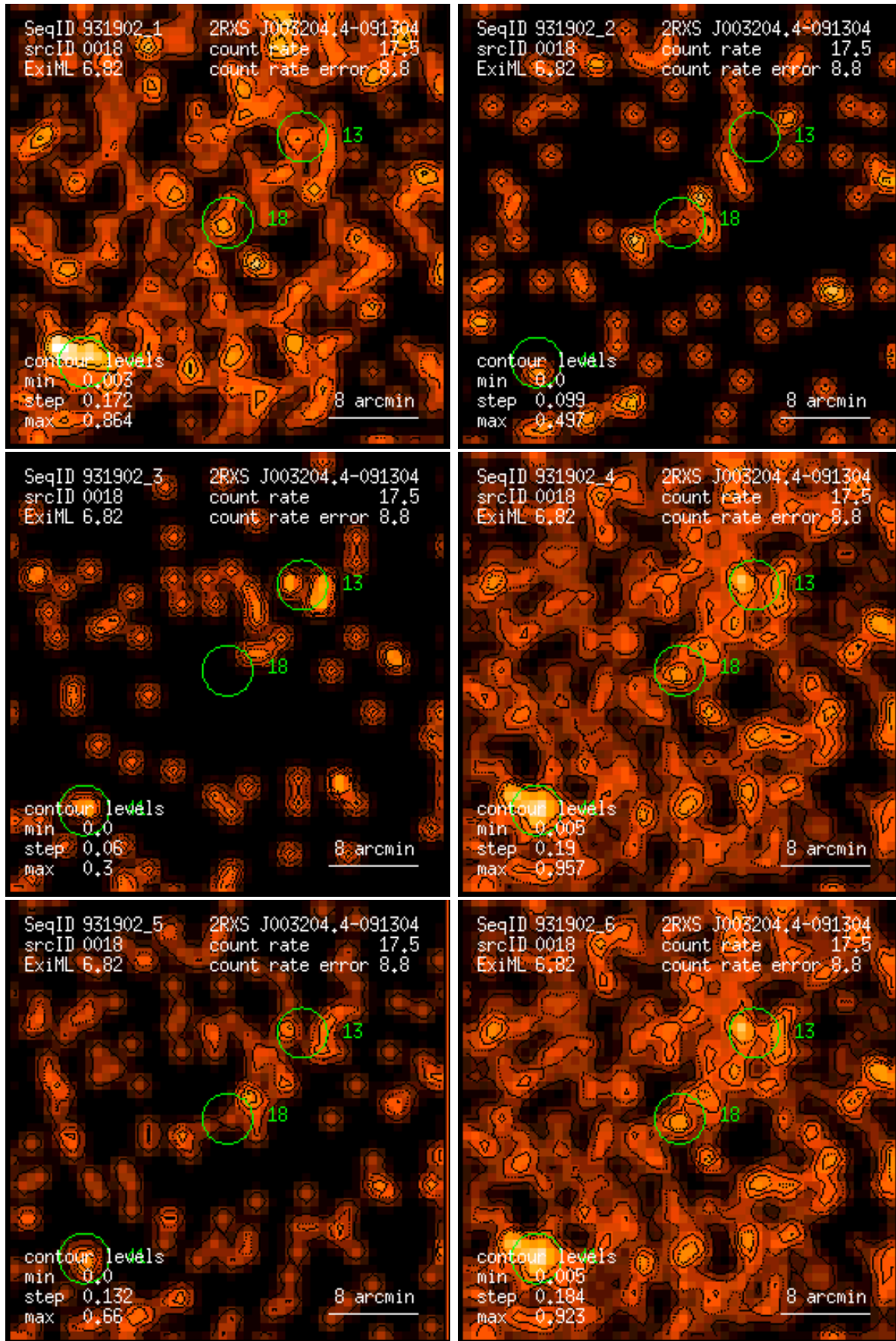
Figure 18: RASS 931902: detection 0018: band rate images, Gaussian filter: (1) PSPC channels 11 – 41, (2) 52 – 90, (3) 91 – 201, (4) 11 – 235, (5) 52 – 201, (6) 11 – 201. Broad band rates in counts/ks. Band rate contour levels in counts/ks/arcmin 2 .
