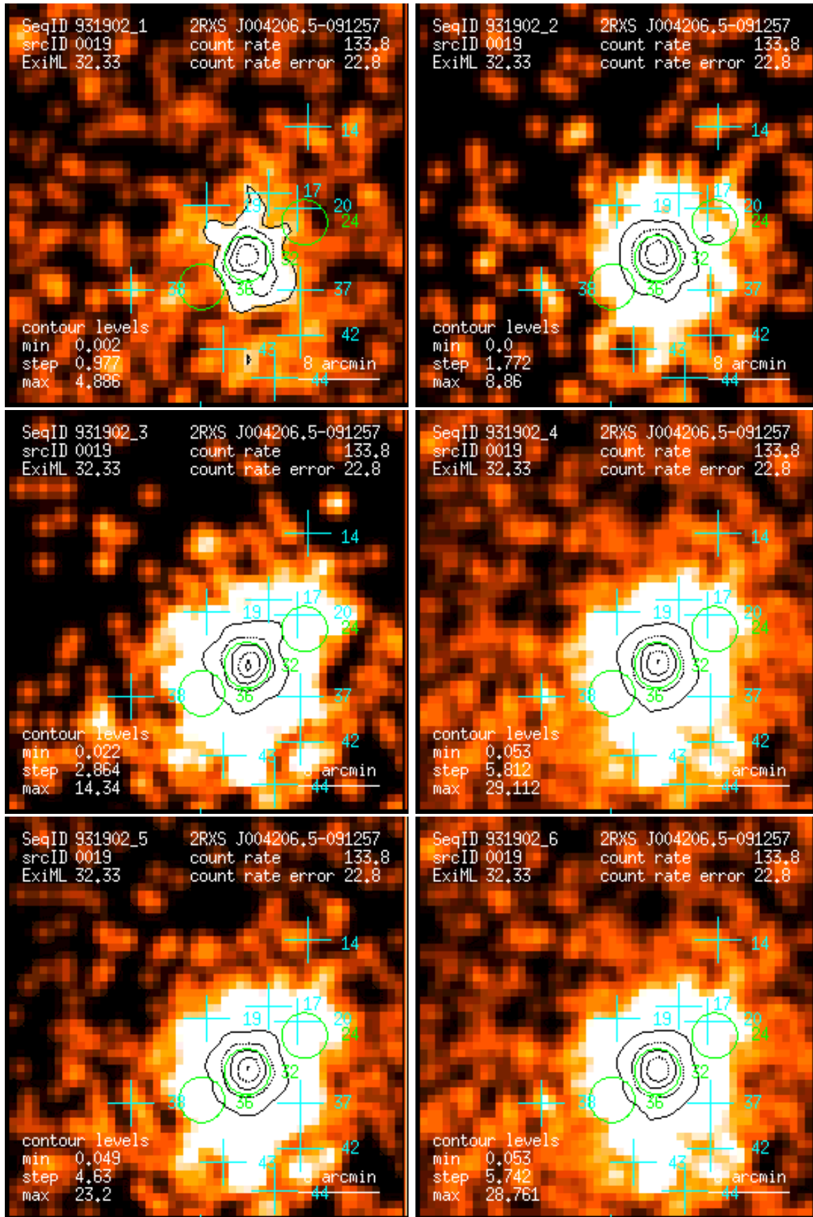
Figure 19: RASS 931902: detection 0019: band rate images, Gaussian filter: (1) PSPC channels 11 – 41, (2) 52 – 90, (3) 91 – 201, (4) 11 – 235, (5) 52 – 201, (6) 11 – 201. Broad band rates in counts/ks. Band rate contour levels in counts/ks/arcmin 2 .
