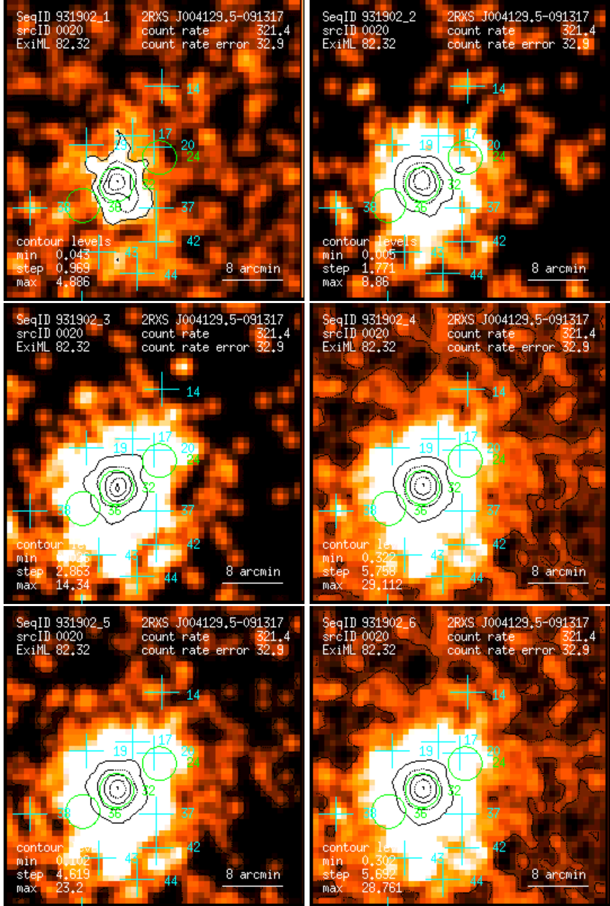
Figure 20: RASS 931902: detection 0020: band rate images, Gaussian filter: (1) PSPC channels 11 – 41, (2) 52 – 90, (3) 91 – 201, (4) 11 – 235, (5) 52 – 201, (6) 11 – 201. Broad band rates in counts/ks. Band rate contour levels in counts/ks/arcmin 2 .
