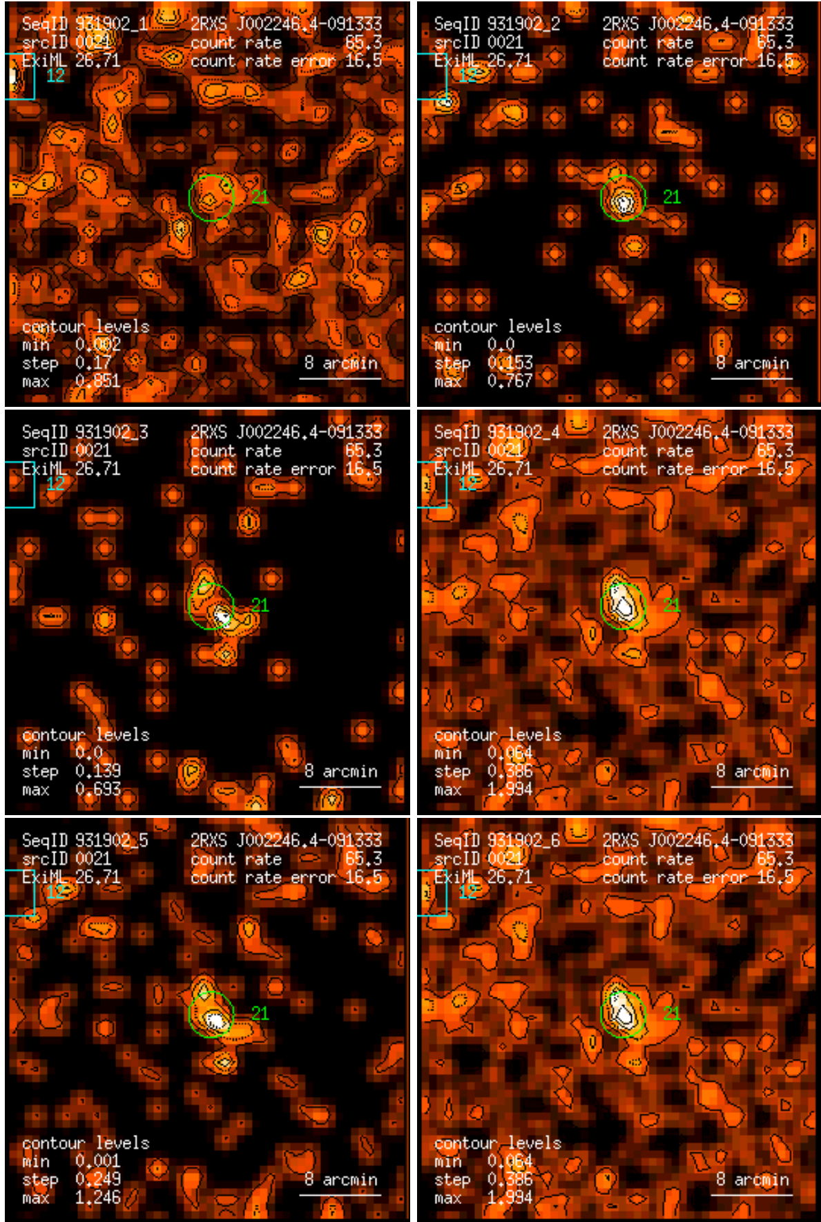
Figure 21: RASS 931902: detection 0021: band rate images, Gaussian filter: (1) PSPC channels 11 – 41, (2) 52 – 90, (3) 91 – 201, (4) 11 – 235, (5) 52 – 201, (6) 11 – 201. Broad band rates in counts/ks. Band rate contour levels in counts/ks/arcmin 2 .
