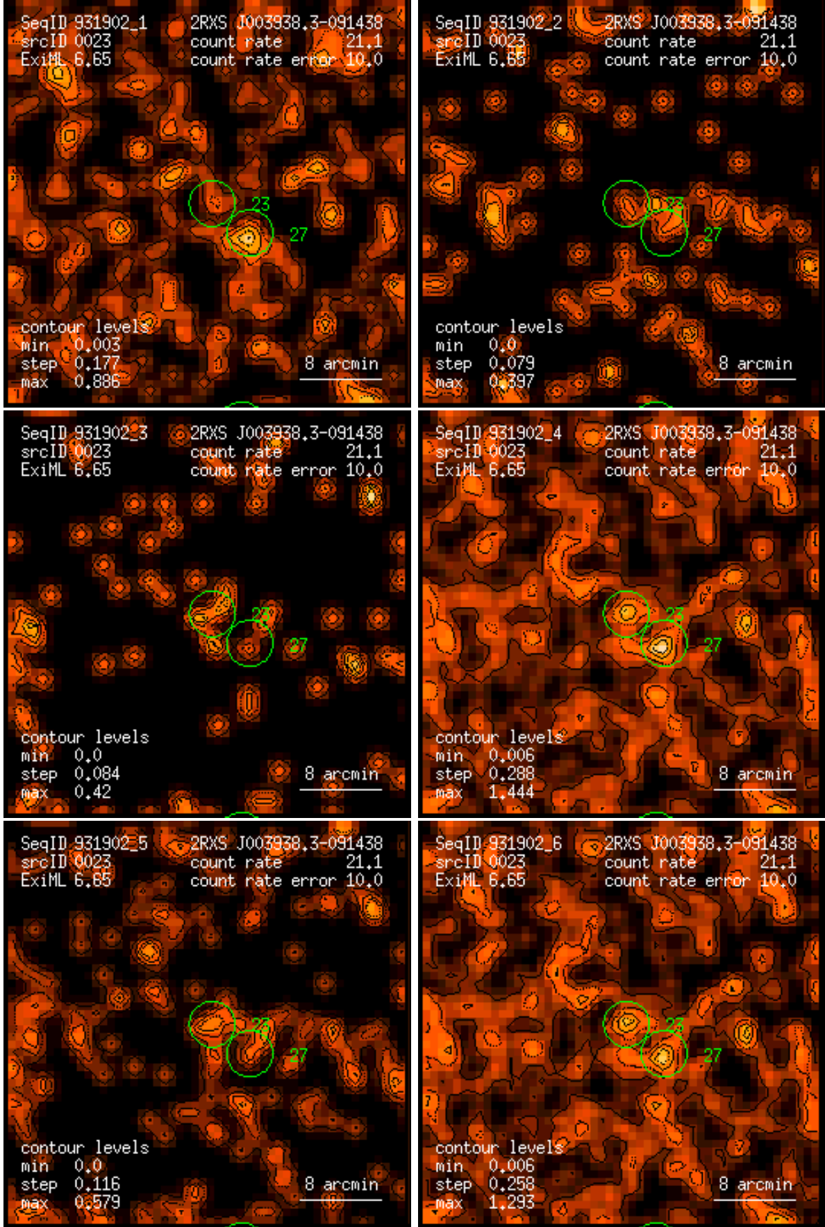
Figure 23: RASS 931902: detection 0023: band rate images, Gaussian filter: (1) PSPC channels 11 – 41, (2) 52 – 90, (3) 91 – 201, (4) 11 – 235, (5) 52 – 201, (6) 11 – 201. Broad band rates in counts/ks. Band rate contour levels in counts/ks/arcmin 2 .
