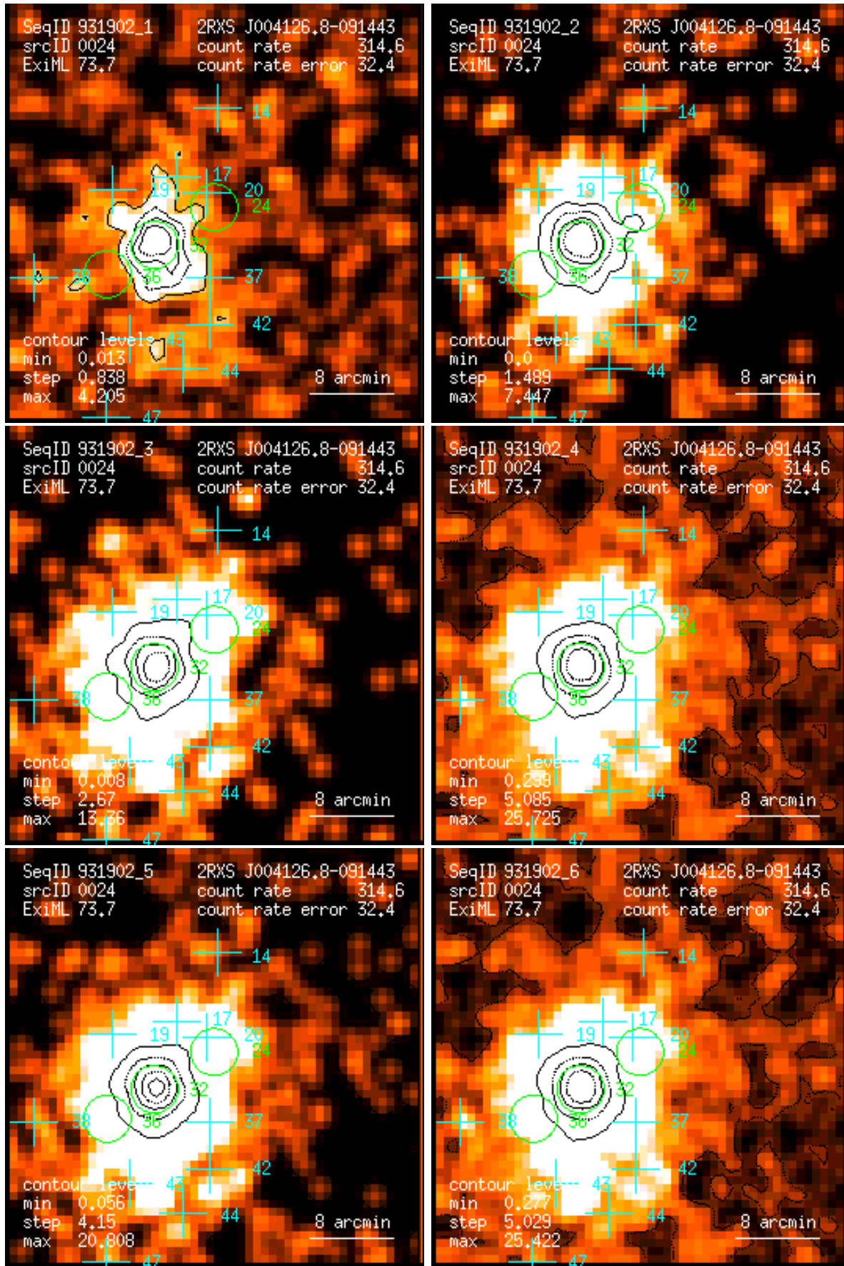
Figure 24: RASS 931902: detection 0024: band rate images, Gaussian filter: (1) PSPC channels 11 – 41, (2) 52 – 90, (3) 91 – 201, (4) 11 – 235, (5) 52 – 201, (6) 11 – 201. Broad band rates in counts/ks. Band rate contour levels in counts/ks/arcmin 2 .
