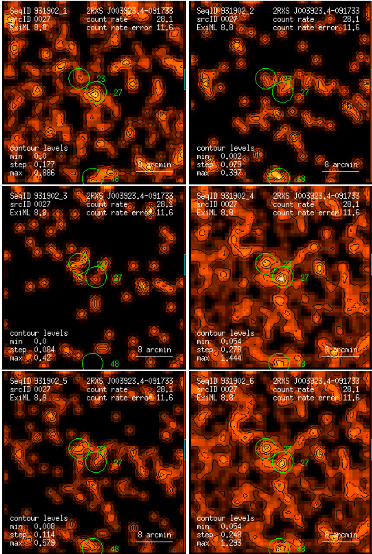
Figure 27: RASS 931902: detection 0027: band rate images, Gaussian filter: (1) PSPC channels 11 – 41, (2) 52 – 90, (3) 91 – 201, (4) 11 – 235, (5) 52 – 201, (6) 11 – 201. Broad band rates in counts/ks. Band rate contour levels in counts/ks/arcmin 2 .
