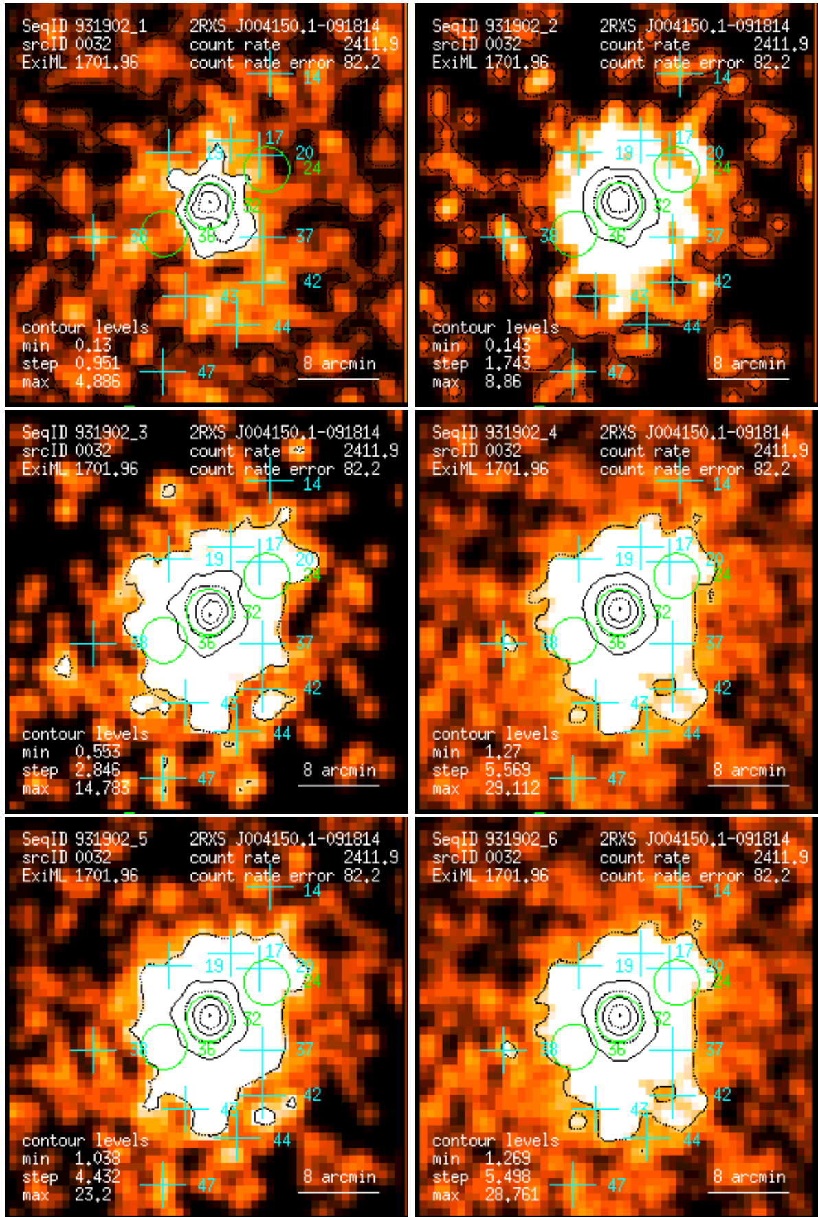
Figure 32: RASS 931902: detection 0032: band rate images, Gaussian filter: (1) PSPC channels 11 – 41, (2) 52 – 90, (3) 91 – 201, (4) 11 – 235, (5) 52 – 201, (6) 11 – 201. Broad band rates in counts/ks. Band rate contour levels in counts/ks/arcmin 2 .
