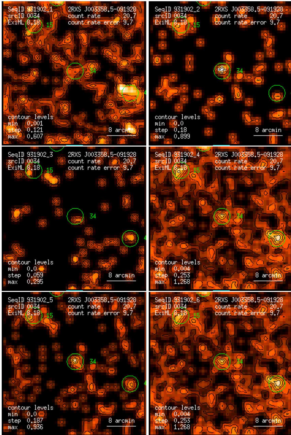
Figure 34: RASS 931902: detection 0034: band rate images, Gaussian filter: (1) PSPC channels 11 – 41, (2) 52 – 90, (3) 91 – 201, (4) 11 – 235, (5) 52 – 201, (6) 11 – 201. Broad band rates in counts/ks. Band rate contour levels in counts/ks/arcmin 2 .
