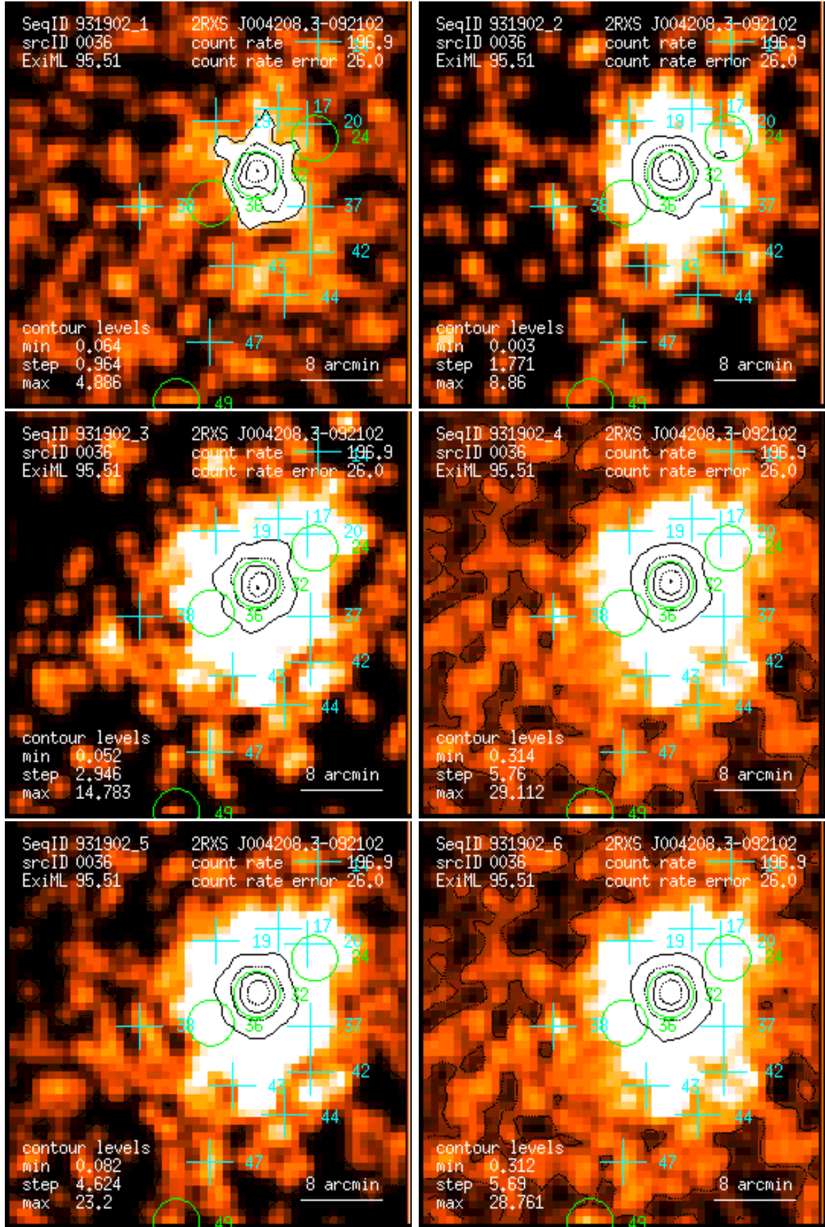
Figure 36: RASS 931902: detection 0036: band rate images, Gaussian filter: (1) PSPC channels 11 – 41, (2) 52 – 90, (3) 91 – 201, (4) 11 – 235, (5) 52 – 201, (6) 11 – 201. Broad band rates in counts/ks. Band rate contour levels in counts/ks/arcmin 2 .
