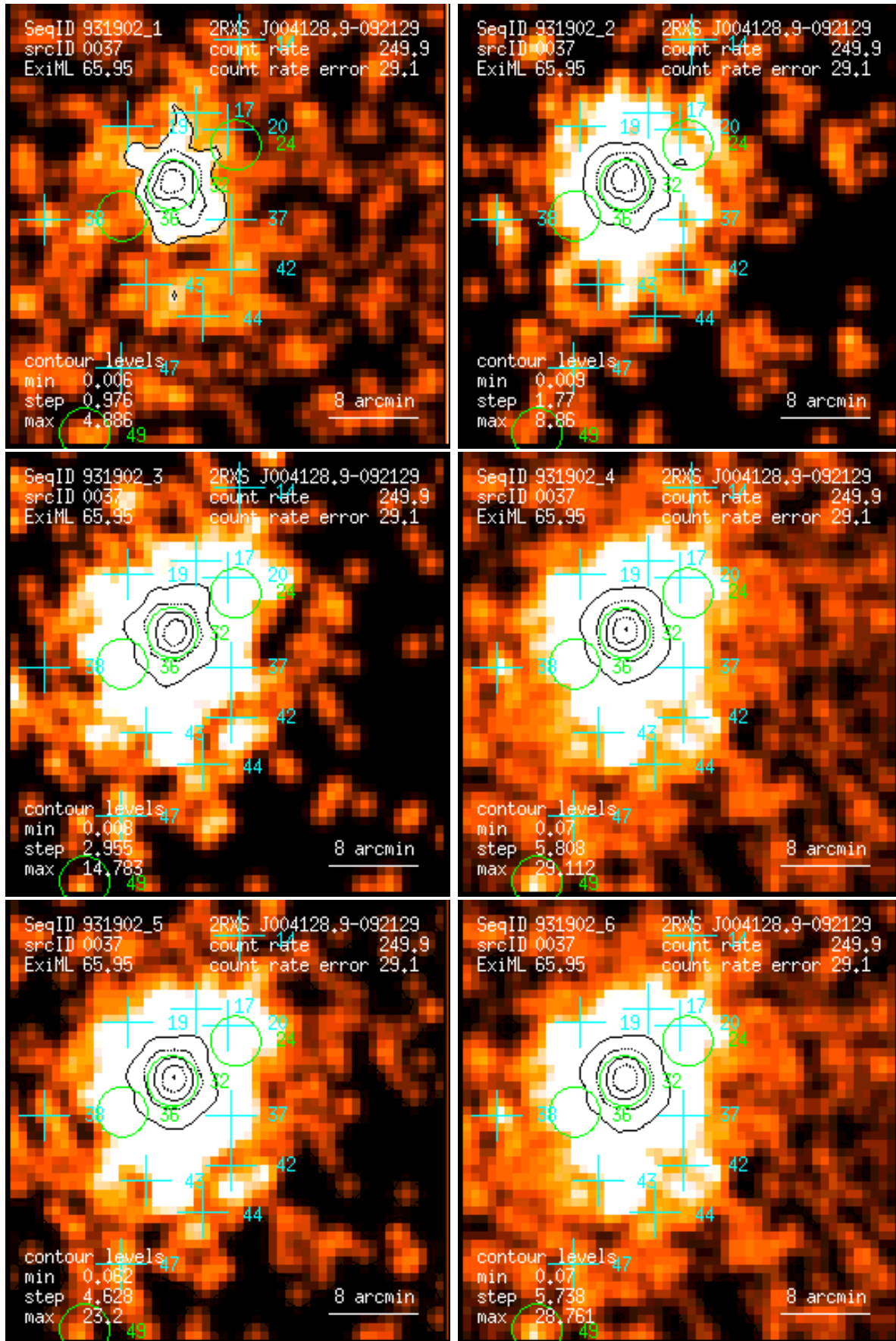
Figure 37: RASS 931902: detection 0037: band rate images, Gaussian filter: (1) PSPC channels 11 – 41, (2) 52 – 90, (3) 91 – 201, (4) 11 – 235, (5) 52 – 201, (6) 11 – 201. Broad band rates in counts/ks. Band rate contour levels in counts/ks/arcmin 2 .
