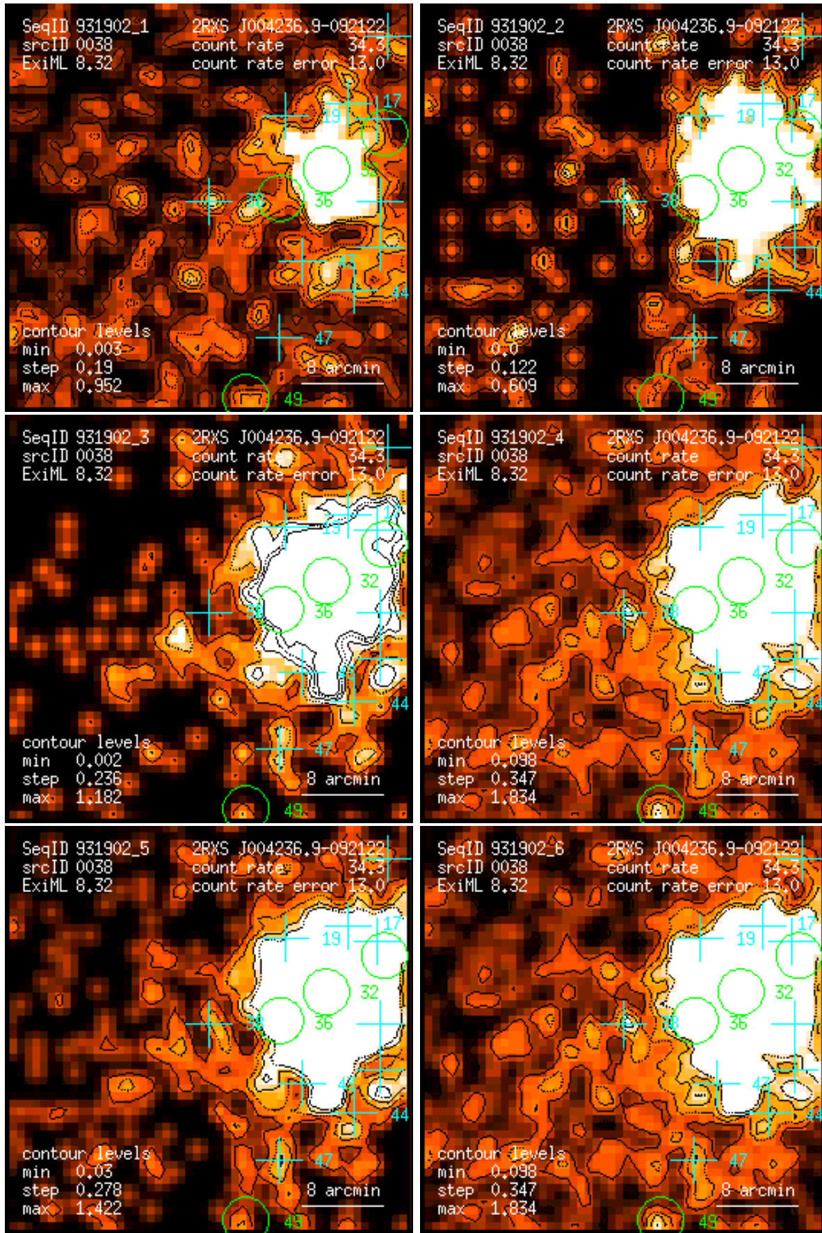
Figure 38: RASS 931902: detection 0038: band rate images, Gaussian filter: (1) PSPC channels 11 – 41, (2) 52 – 90, (3) 91 – 201, (4) 11 – 235, (5) 52 – 201, (6) 11 – 201. Broad band rates in counts/ks. Band rate contour levels in counts/ks/arcmin 2 .
