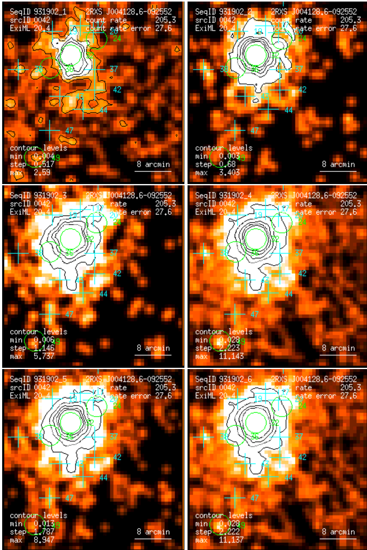
Figure 42: RASS 931902: detection 0042: band rate images, Gaussian filter: (1) PSPC channels 11 – 41, (2) 52 – 90, (3) 91 – 201, (4) 11 – 235, (5) 52 – 201, (6) 11 – 201. Broad band rates in counts/ks. Band rate contour levels in counts/ks/arcmin 2 .
