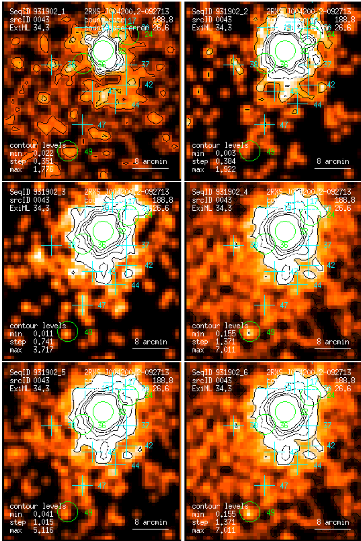
Figure 43: RASS 931902: detection 0043: band rate images, Gaussian filter: (1) PSPC channels 11 – 41, (2) 52 – 90, (3) 91 – 201, (4) 11 – 235, (5) 52 – 201, (6) 11 – 201. Broad band rates in counts/ks. Band rate contour levels in counts/ks/arcmin 2 .
