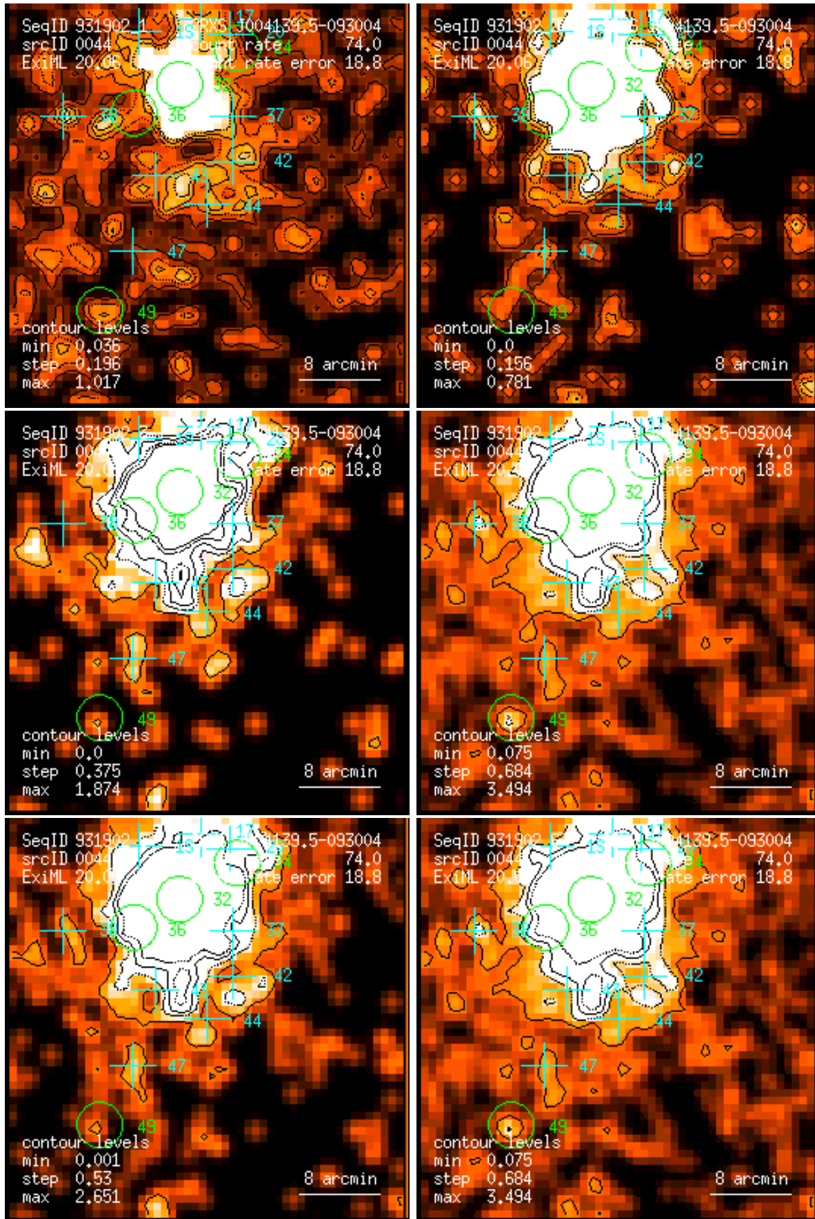
Figure 44: RASS 931902: detection 0044: band rate images, Gaussian filter: (1) PSPC channels 11 – 41, (2) 52 – 90, (3) 91 – 201, (4) 11 – 235, (5) 52 – 201, (6) 11 – 201. Broad band rates in counts/ks. Band rate contour levels in counts/ks/arcmin 2 .
