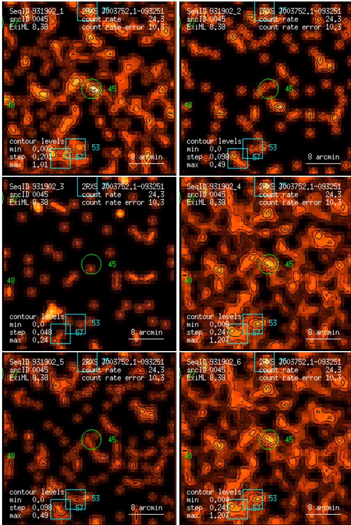
Figure 45: RASS 931902: detection 0045: band rate images, Gaussian filter: (1) PSPC channels 11 – 41, (2) 52 – 90, (3) 91 – 201, (4) 11 – 235, (5) 52 – 201, (6) 11 – 201. Broad band rates in counts/ks. Band rate contour levels in counts/ks/arcmin 2 .
