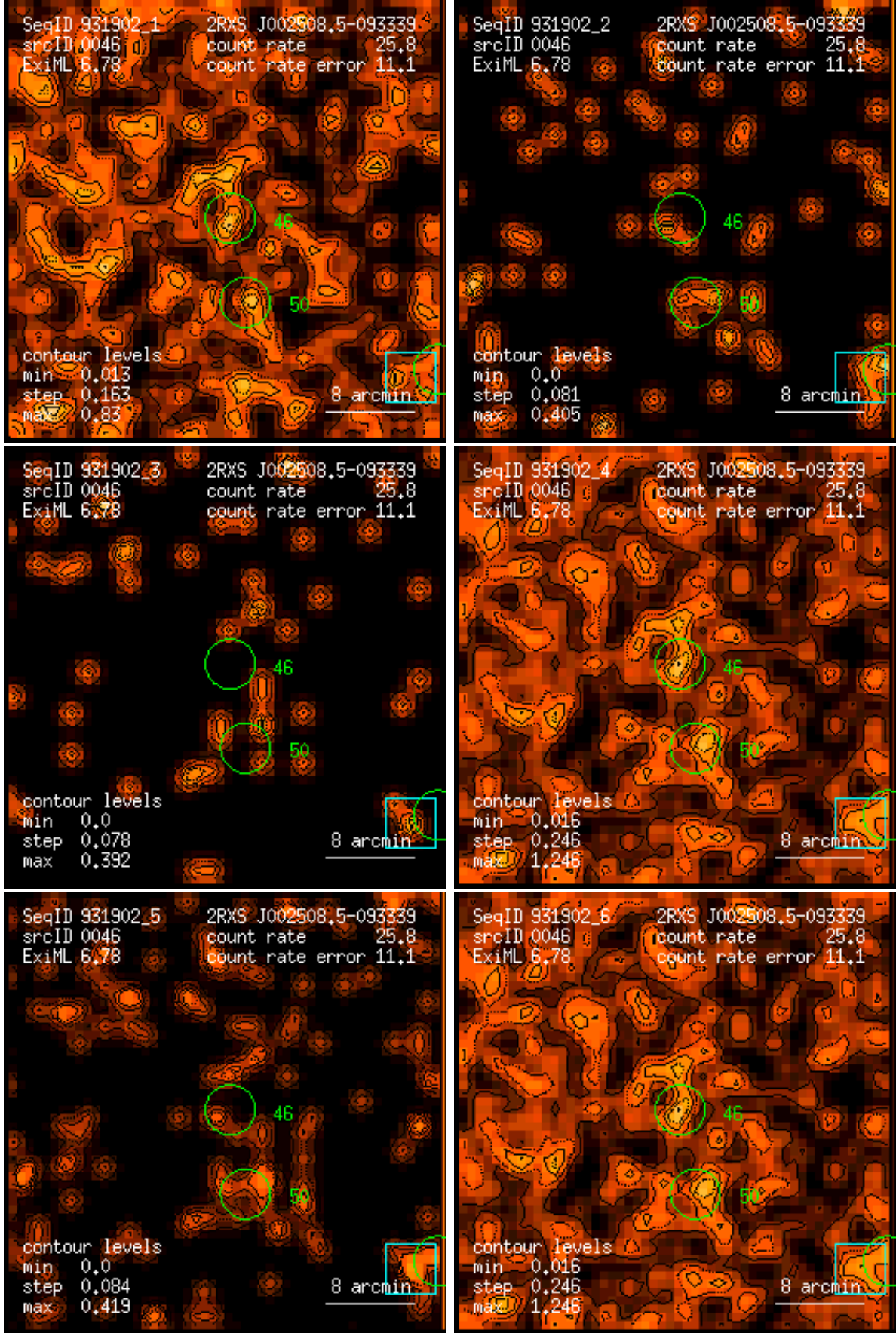
Figure 46: RASS 931902: detection 0046: band rate images, Gaussian filter: (1) PSPC channels 11 – 41, (2) 52 – 90, (3) 91 – 201, (4) 11 – 235, (5) 52 – 201, (6) 11 – 201. Broad band rates in counts/ks. Band rate contour levels in counts/ks/arcmin 2 .
